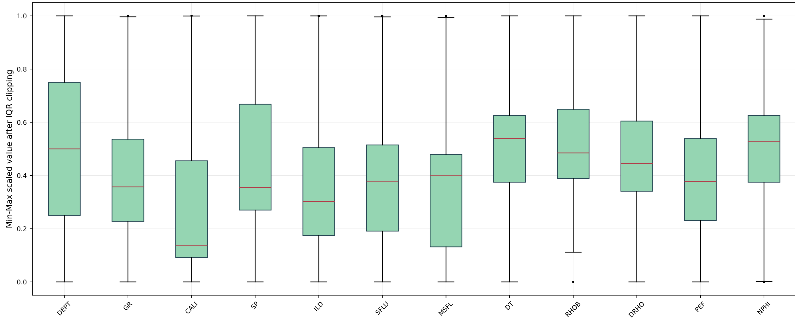
Boxplot for Input-Feature Outliers After IQR Treatment
