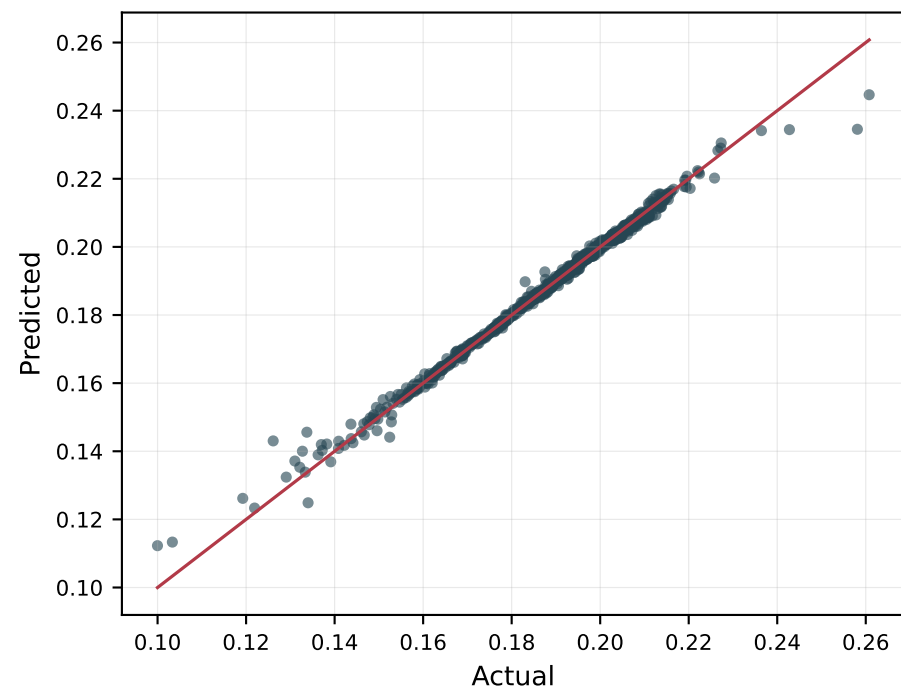
Porosity Random Forest
