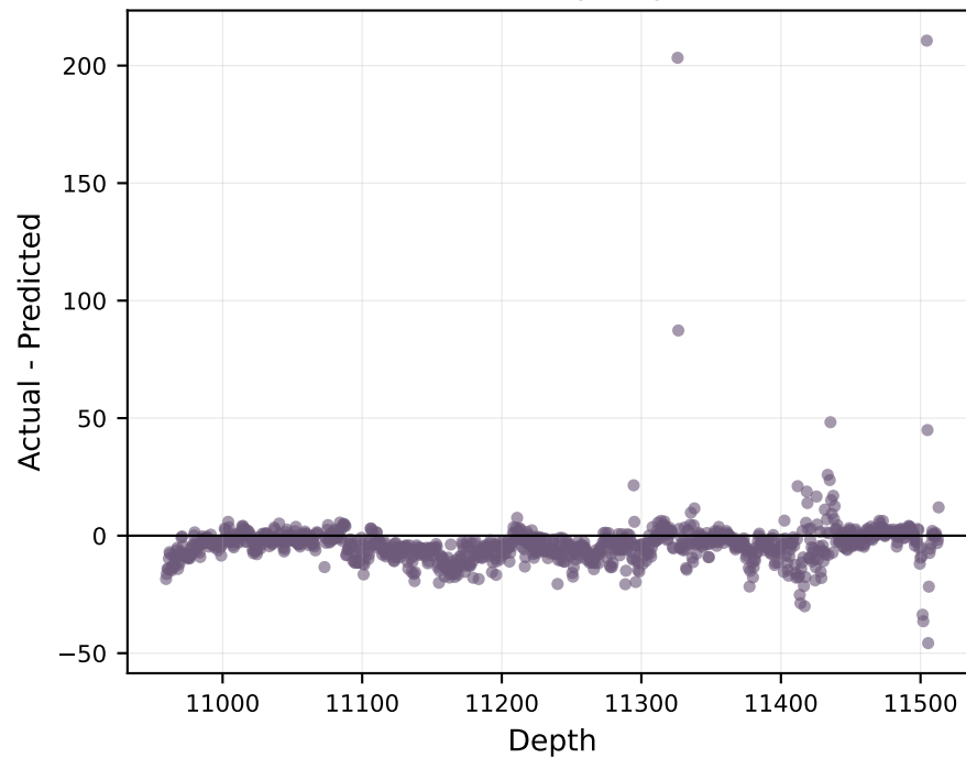
Permeability k Residual by depth
