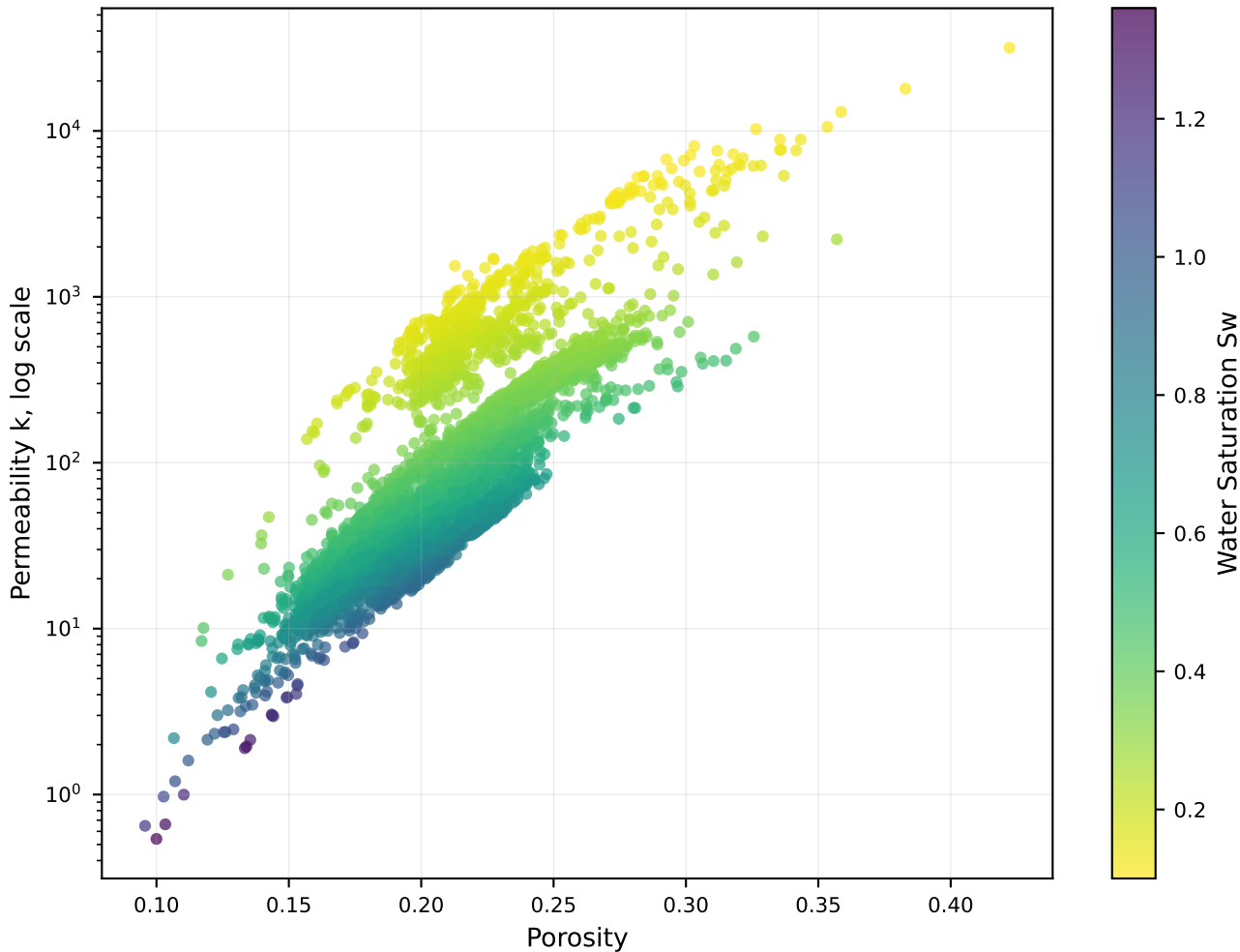
Reservoir Quality Crossplot: Porosity vs Permeability
