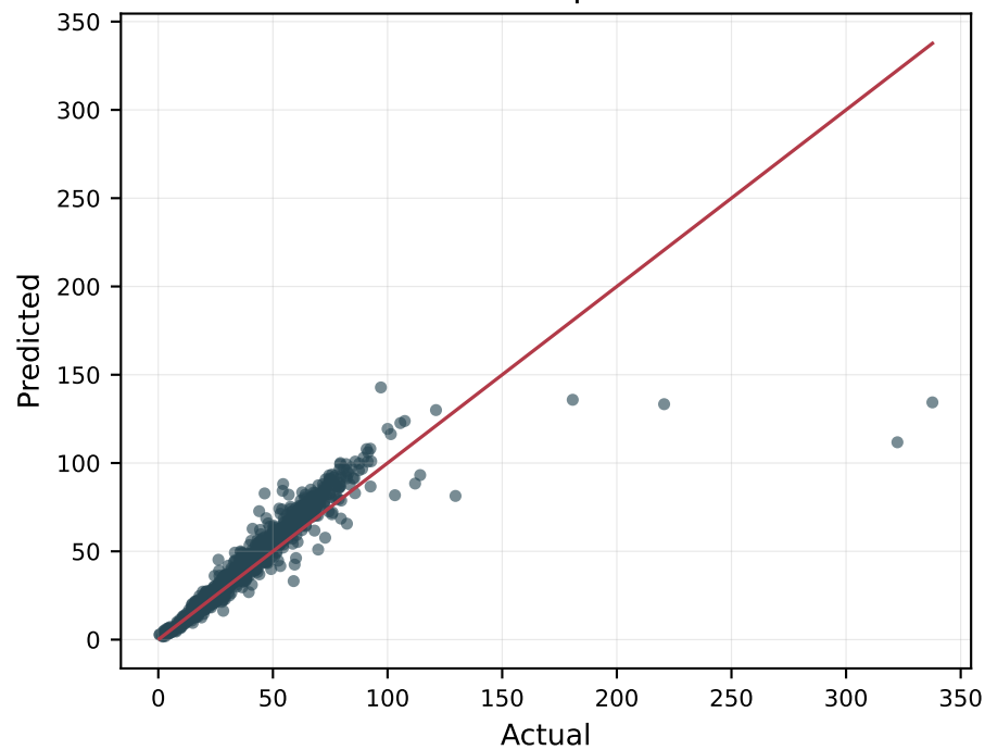
Permeability k ANN Deep MLP
