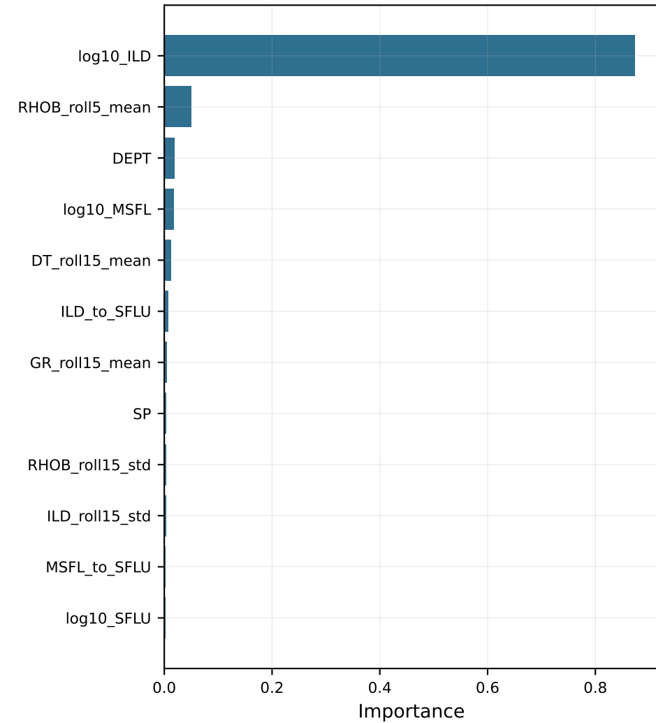
Water Saturation Sw
