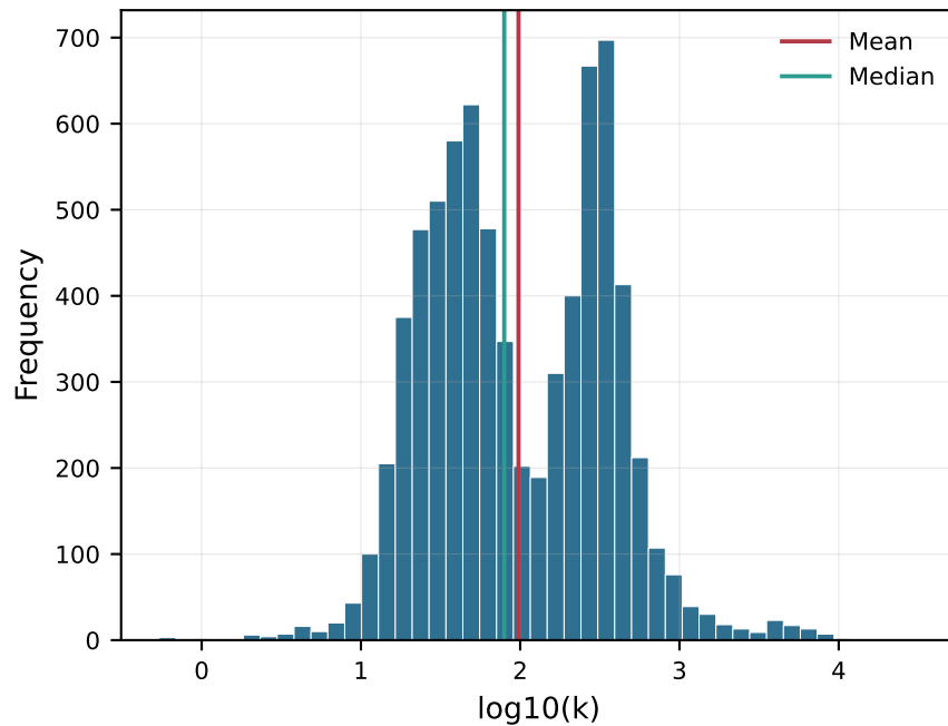
Permeability k
