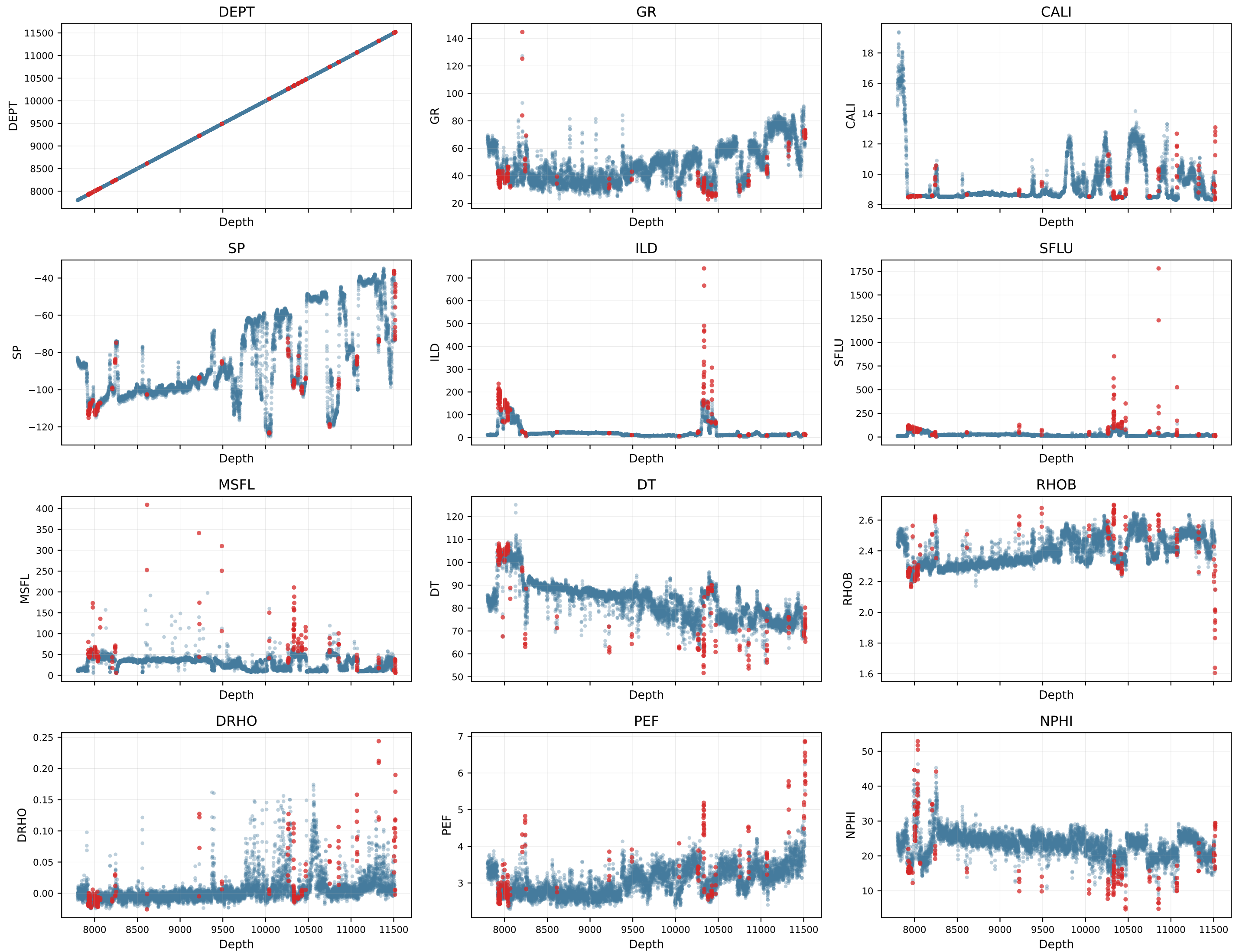
Scattered Plot for Noisy Data Detected by IsolationForest (n = 186)
