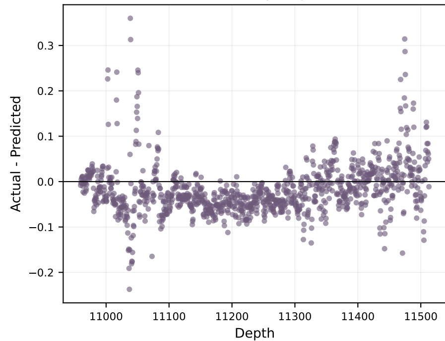
Water Saturation Sw Residual by depth
