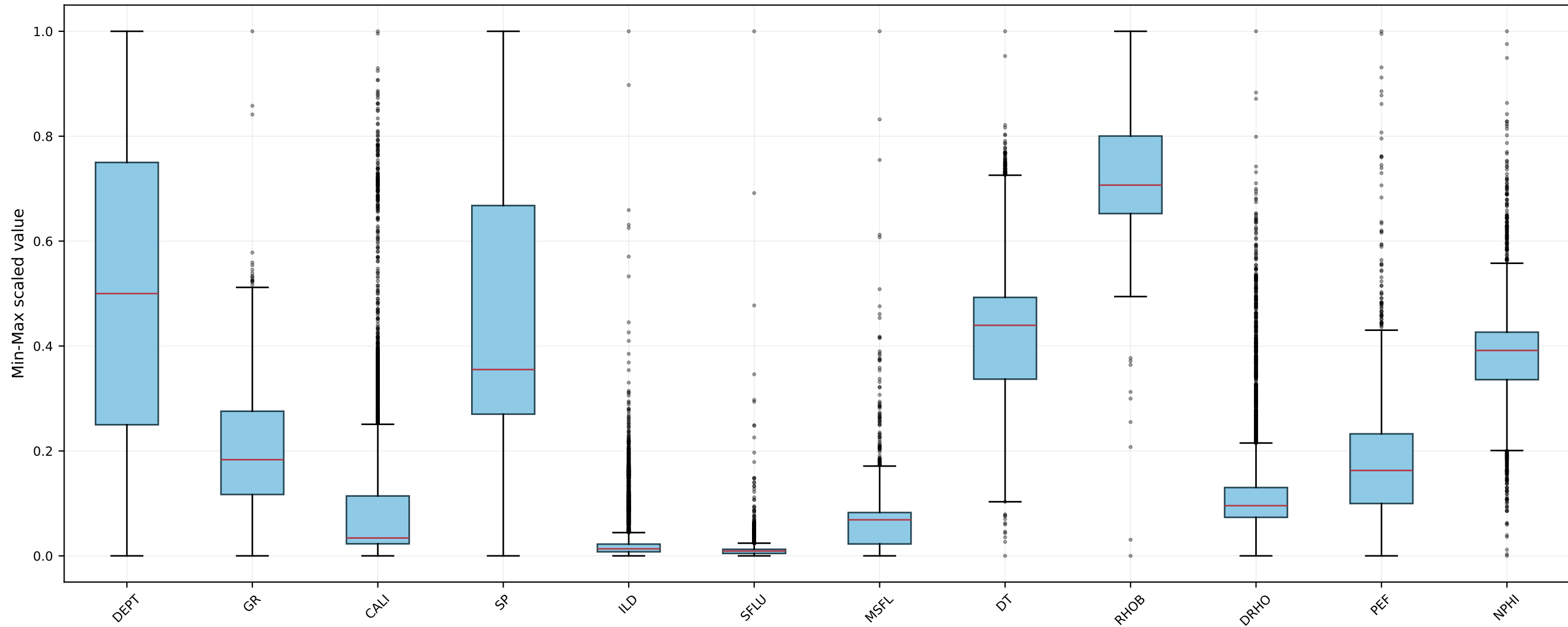
Boxplot for Input-Feature Outliers Before IQR Treatment
