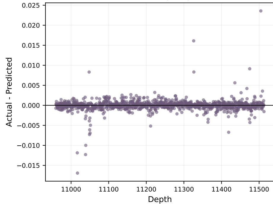
Porosity Residual by depth
