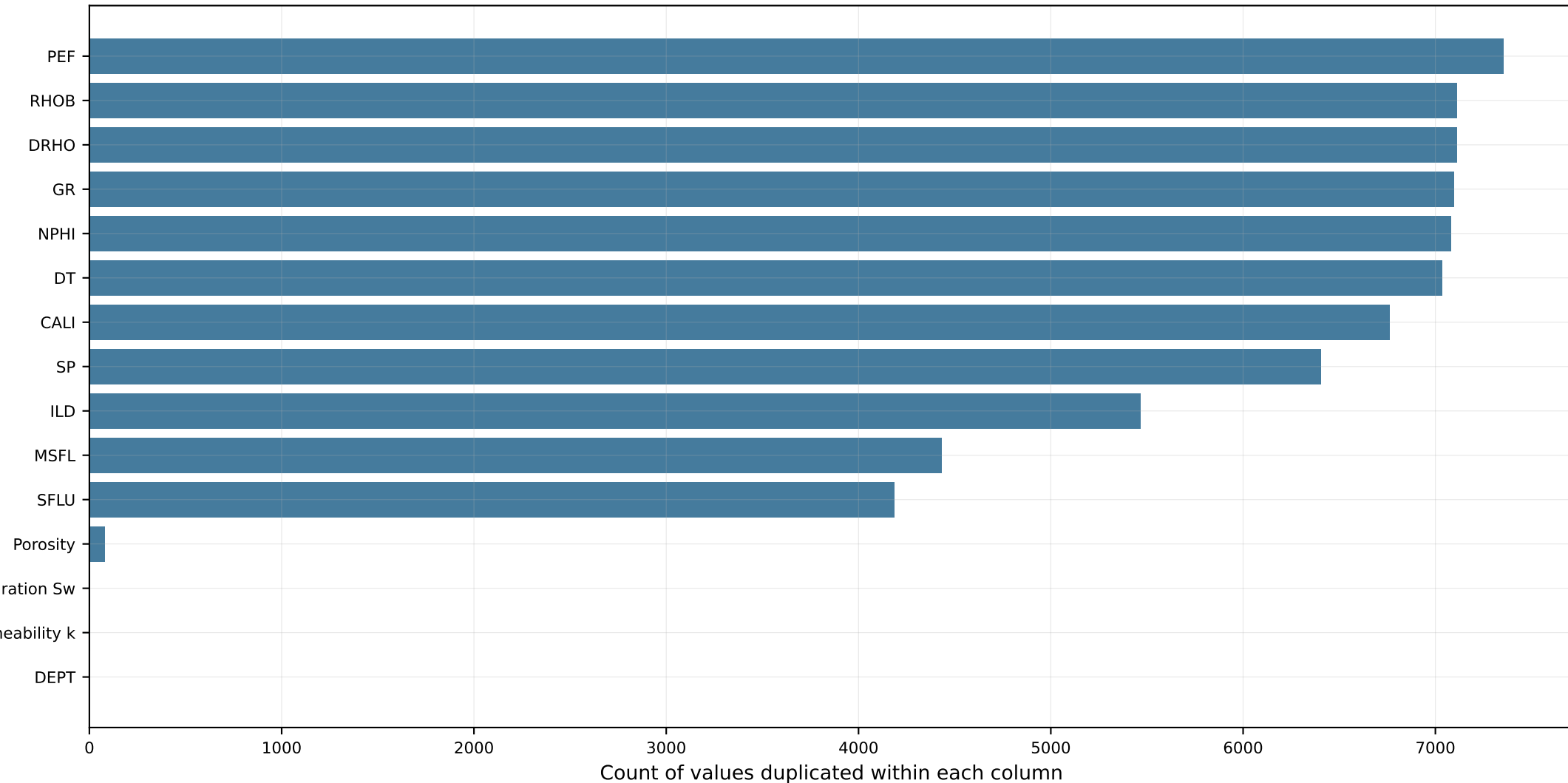
Histogram for Duplicate Data by Column (full-row duplicates = 0)
