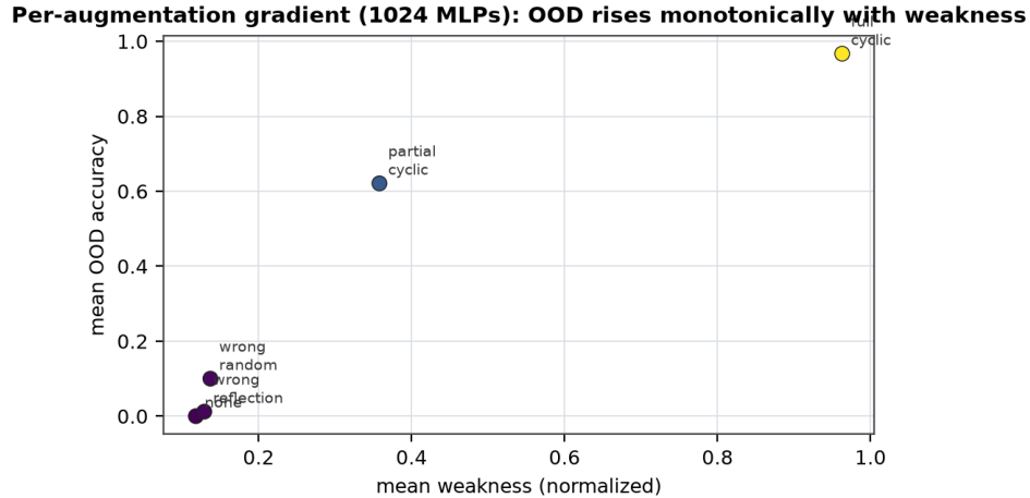
Figure 3. The per-augmentation gradient is monotone in weakness: full-cyclic (orbit completion) saturates at 97% OOD and 0.96 weakness, while none / wrong-reflection collapse to \leq 1\% OOD and \leq 0.13 weakness. Augmentations that approximately respect the symmetry raise weakness and OOD together.
