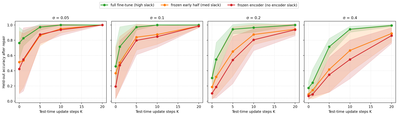
Repair under viability breach: noise classifier head with \sigma , then K test-time updates on held-out paraphrases
