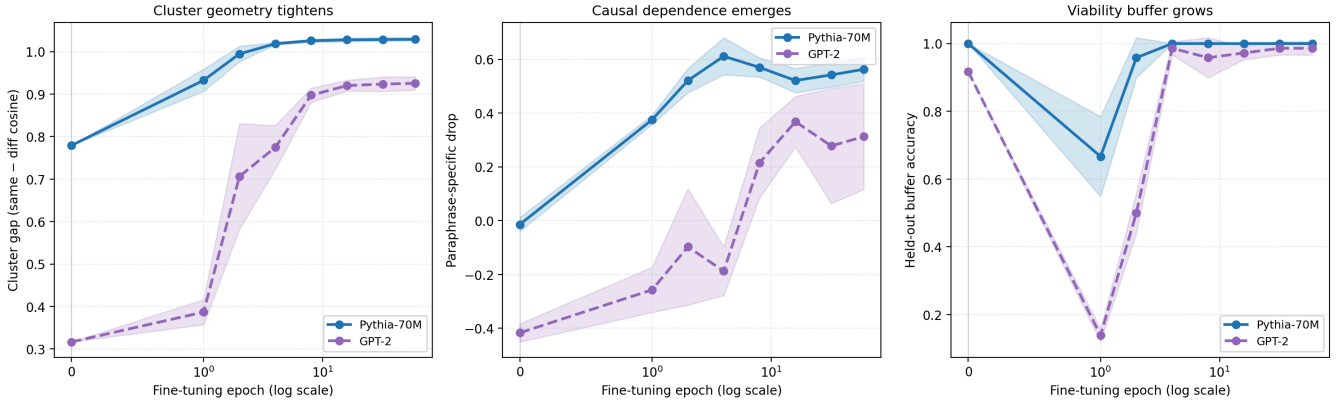
Trajectory of the passive→active transition under full fine-tune (mean ± std across 3 seeds)
