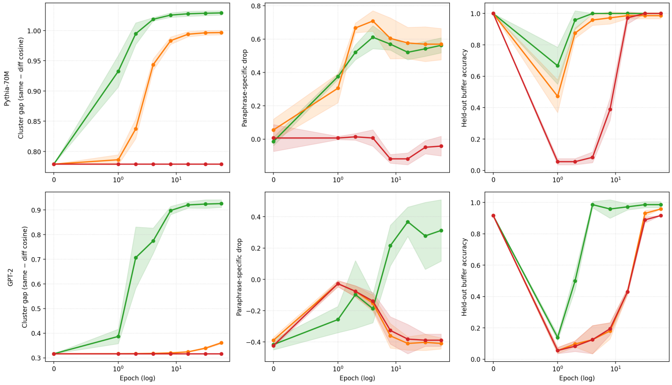
Law of the Stack: lower-layer slack caps the passive→active transition
