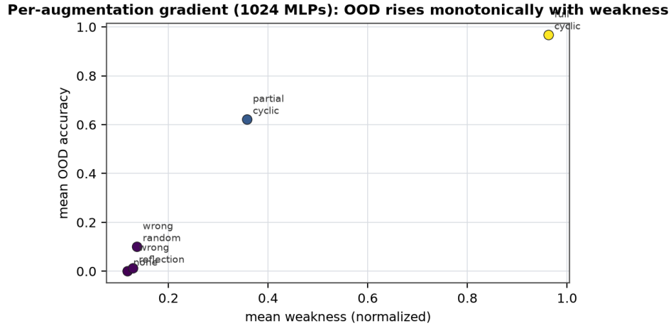
Figure 3. The per-augmentation gradient is monotone in weakness: full-cyclic (orbit completion) saturates at 97% OOD and 0.96 weakness, while none / wrong-reflection collapse to \leq 1\% OOD and \leq 0.13 weakness. Augmentations that approximately respect the symmetry raise weakness and OOD together.
