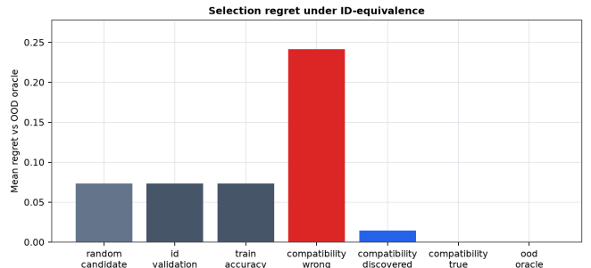
Figure 1: Semantic selector performance. The main paper uses this as the headline visual because it is the closest deployment analogue: choose among ID-equivalent candidates before seeing OOD labels.
