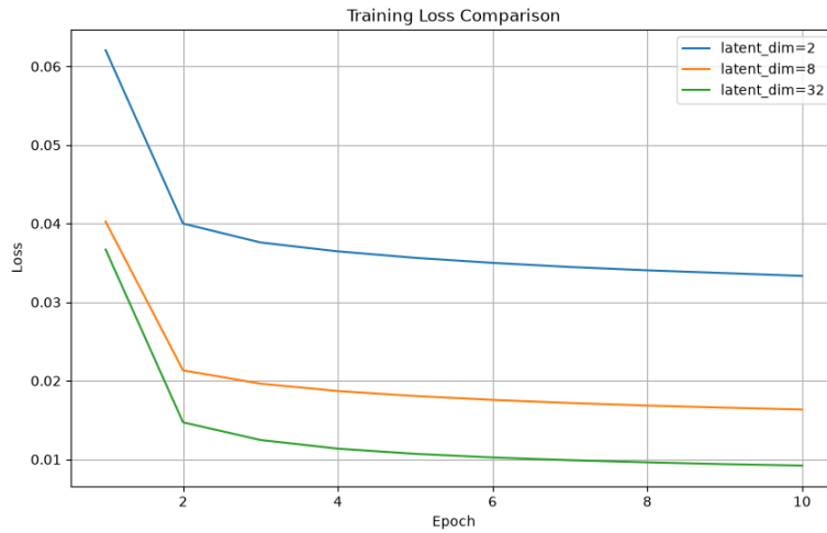
Figure 1: Perbandingan training loss antar latent dimension
