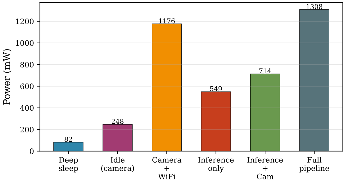
ESP32-S3 Power Consumption by Operating Scenario
