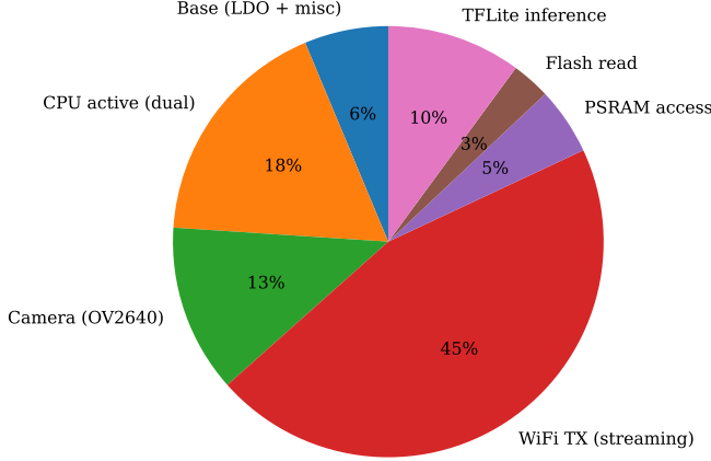
Power Breakdown — Full Pipeline
