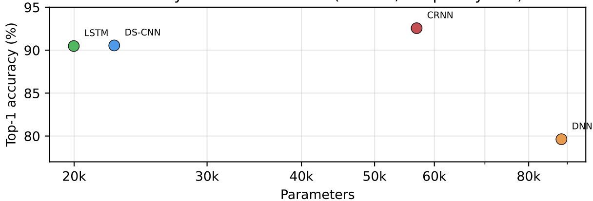
Accuracy versus model size (float32, Raspberry Pi 5)
