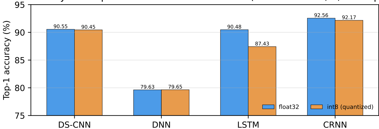
Accuracy over Speech Commands v2 test set (10 commands, 4,074 clips)
