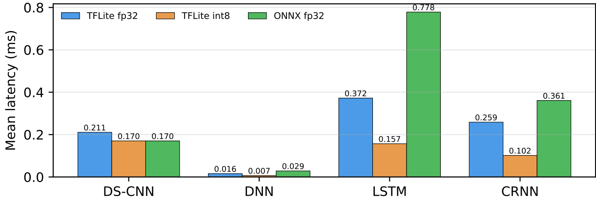
Inference latency by model and runtime (Raspberry Pi 5)
