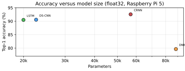
Fig. 3. Top-1 accuracy versus parameter count (float32). The CRNN reaches the highest accuracy with 56.8k parameters, while the dense network spends the most parameters for the lowest accuracy.
