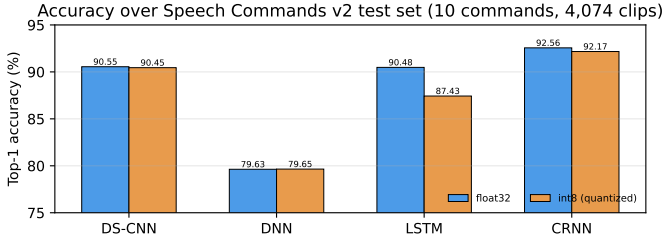
Fig. 1. Top-1 accuracy by model, float32 versus int8-quantized TensorFlow Lite. The LSTM is the only architecture for which quantization costs more than half a point. For DS-CNN the int8 bar is the original mixed-precision artifact, not a full-int8 quantization (see Section IV).
