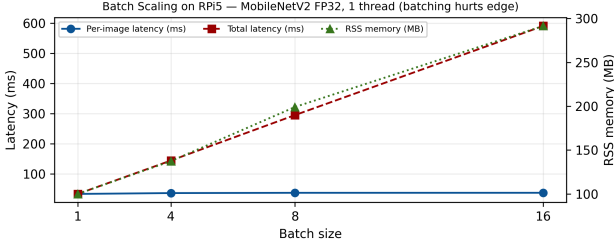
Fig. 2. Batch scaling on RPi5 (MobileNetV2 FP32, 1 thread). Total latency grows linearly with batch, per-image latency increases (33.13 ms at b=1 → 36.92 ms at b=16), and RSS memory grows from 100MB to 292MB. For farm video streaming, batch=1 is optimal.
