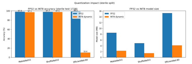
Fig. 4. Quantization impact on the sterile split: accuracy is preserved for MobileNetV2 and ShuffleNetV2 but collapses for EfficientNet-B0 under dynamic INT8, while model size shrinks 3.3–3.7 \times for all three.
