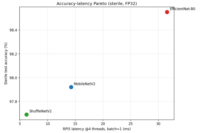
Fig. 3. Accuracy-latency tradeoff (sterile split, FP32). ShuffleNetV2 is fastest (6.19 ms RP15 @4 threads, 97.69%); EfficientNet-B0 is most accurate (98.55%) at 31.56 ms; MobileNetV2 is balanced (97.92%, 14.23 ms).
