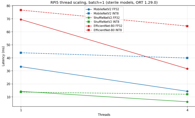
Fig. 2. RP15 thread scaling at batch=1 (sterile models). FP32 (solid) scales from 1 to 4 threads; INT8 (dashed) is flat and slower than FP32 at 4 threads, except ShuffleNetV2 at 1 thread where INT8 is slightly faster.
