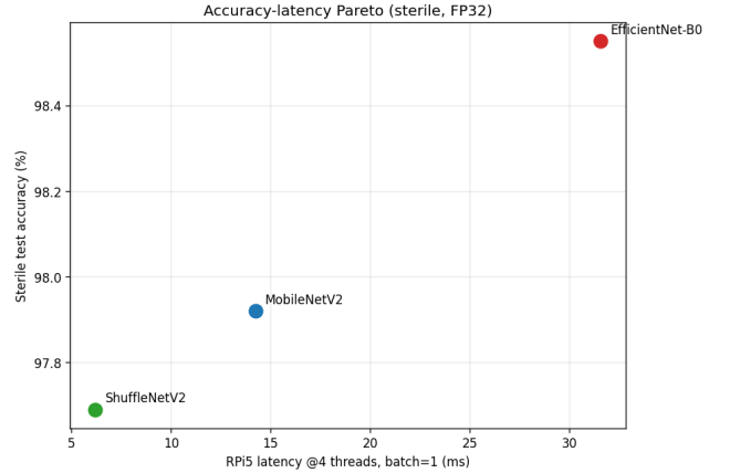
Fig. 3. Accuracy-latency tradeoff (sterile split, FP32). ShuffleNetV2 is fastest (6.19 ms RPi5 @4 threads, 97.69%); EfficientNet-B0 is most accurate (98.55%) at 31.56 ms; MobileNetV2 is balanced (97.92%, 14.23 ms).
