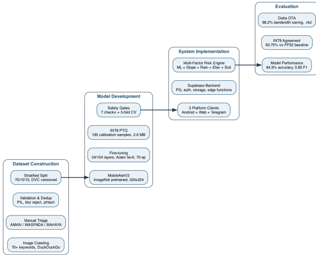
Fig. 2. Research methodology flowchart showing the four-phase pipeline: dataset construction, model development, system implementation, and evaluation
