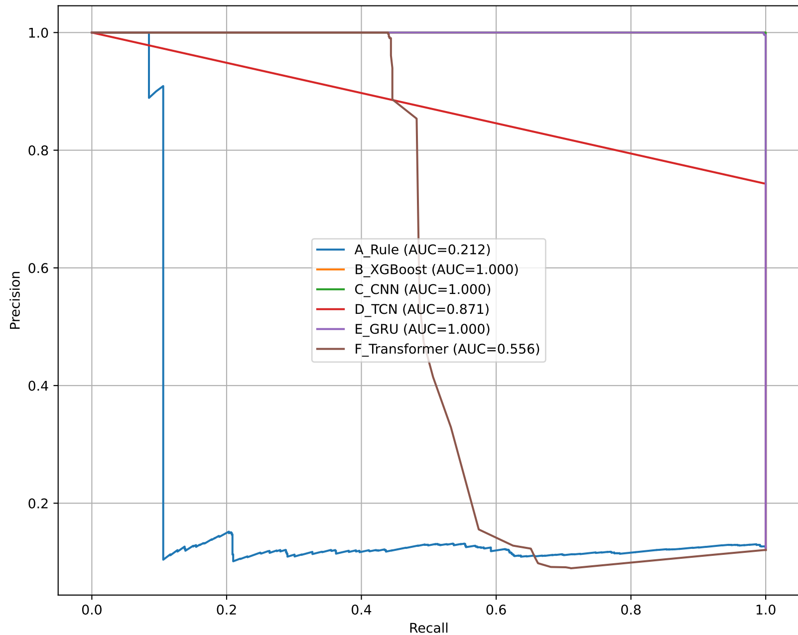
Precision-Recall Curves (Test Set)
