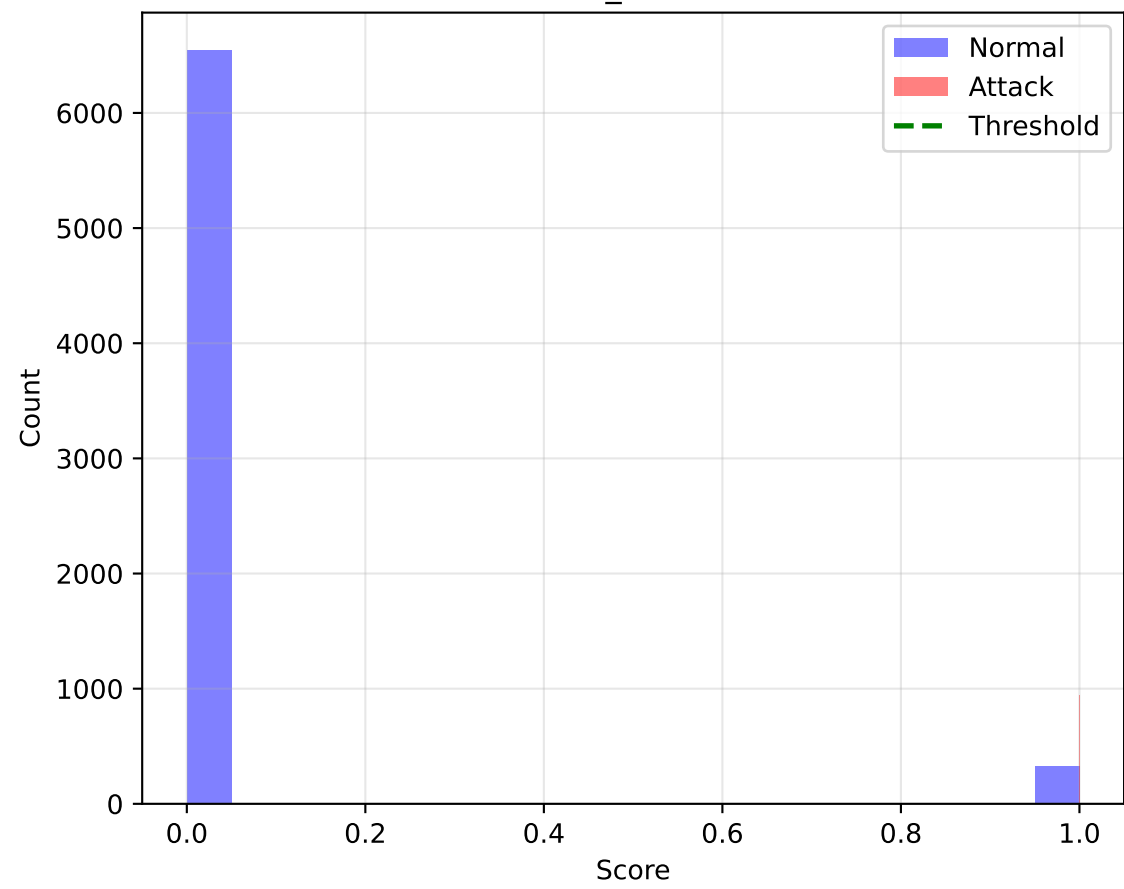
D_TCN
