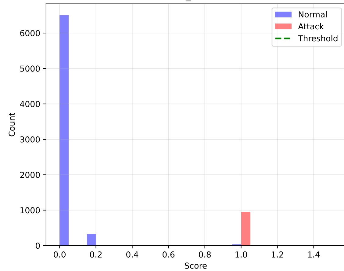
F_Transformer
