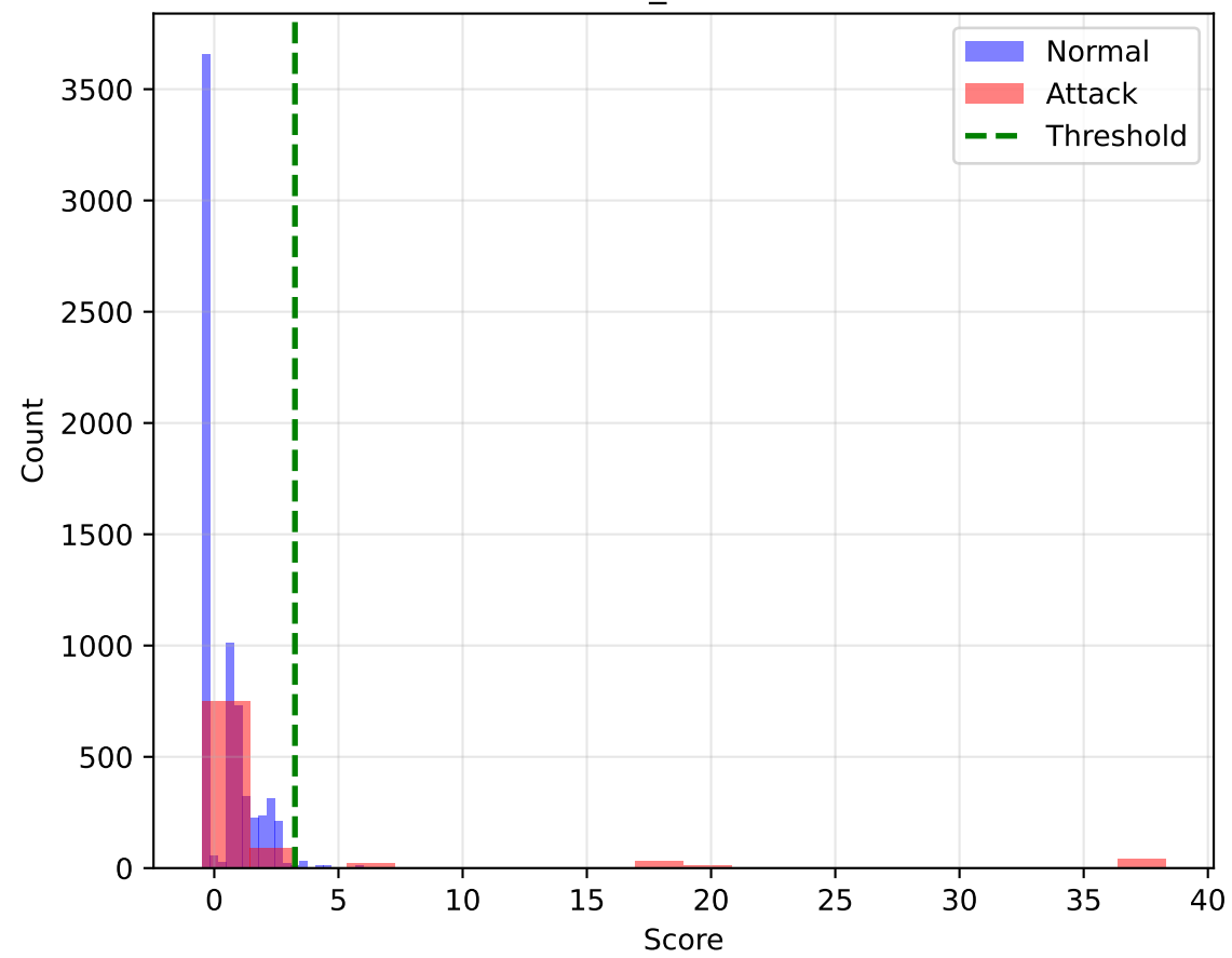
D_TCN
