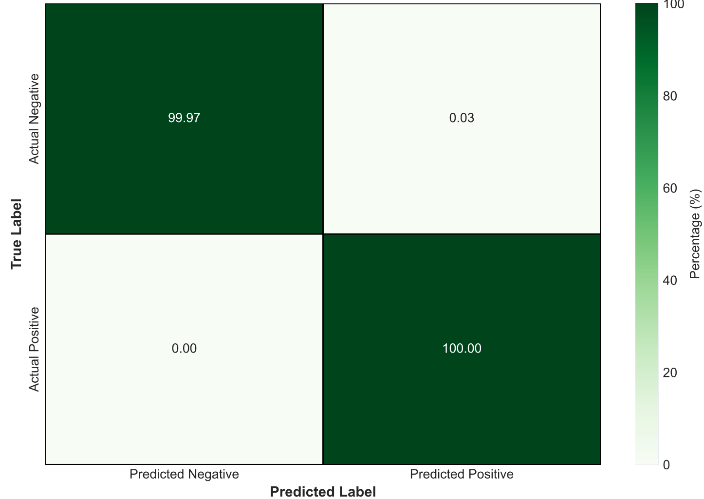
Confusion Matrix - Row Percentages (Threshold=0.8349 @ FPR=1%)
