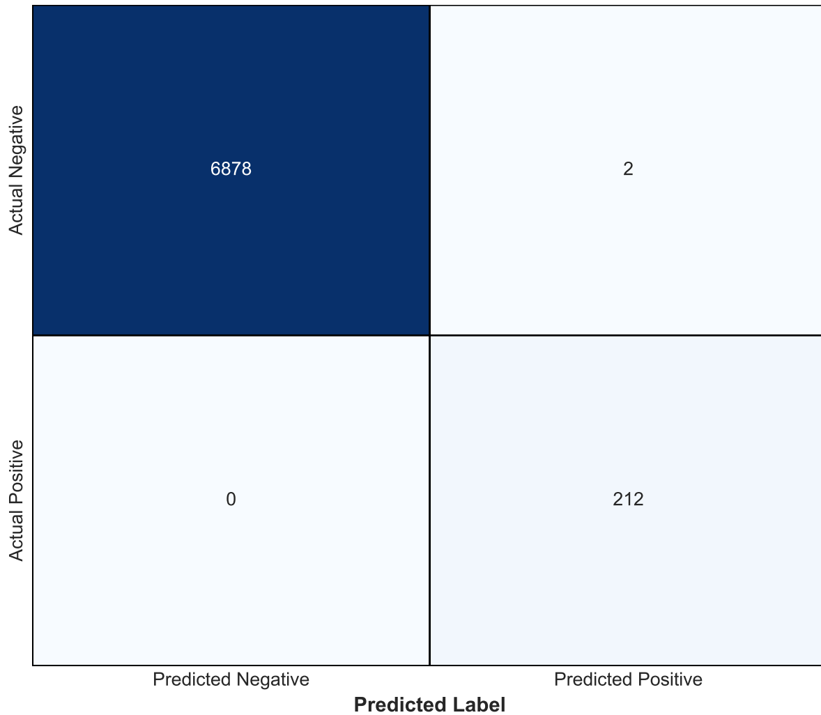
Confusion Matrix - Absolute Counts (Threshold=0.8349 @ FPR=1%)
