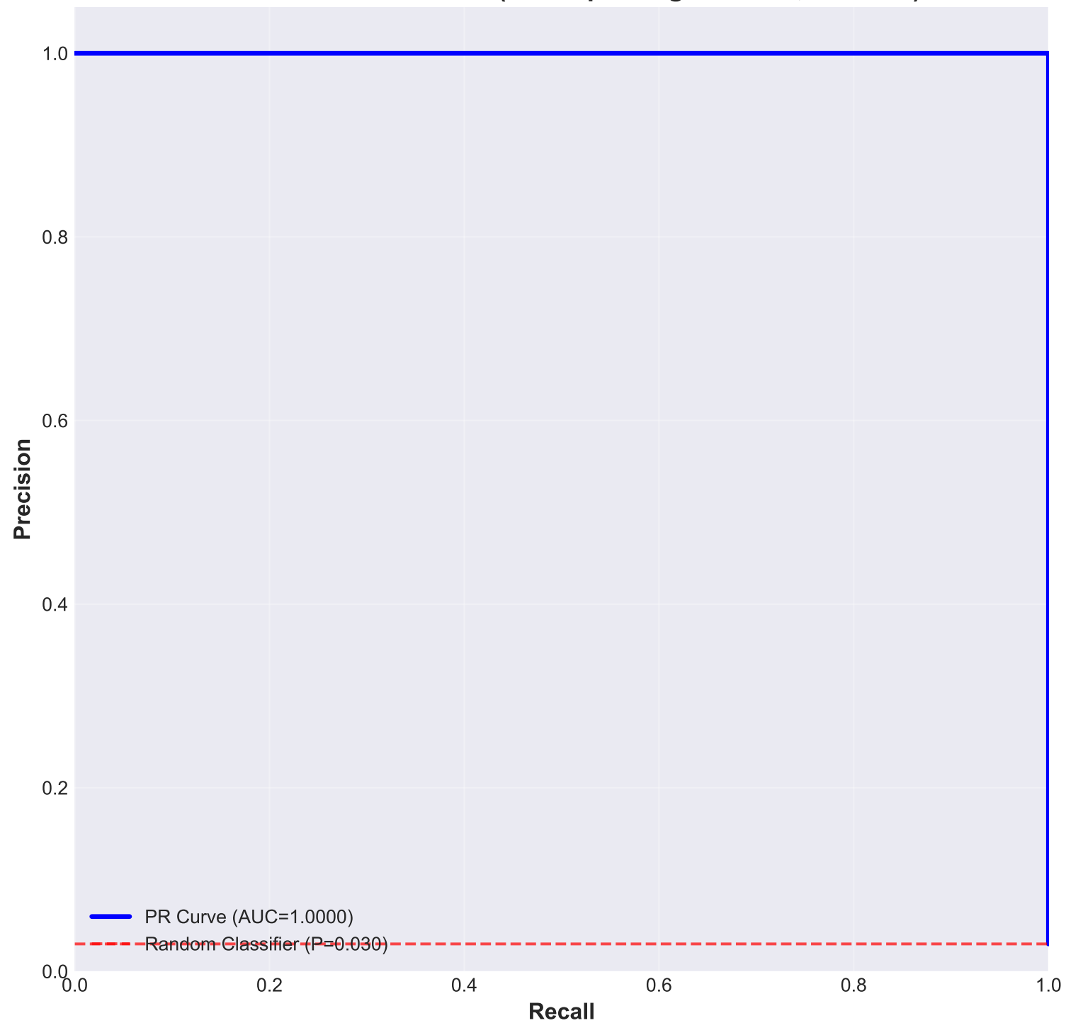
Precision-Recall Curve (GPS Spoofing Detector, Test Set)
