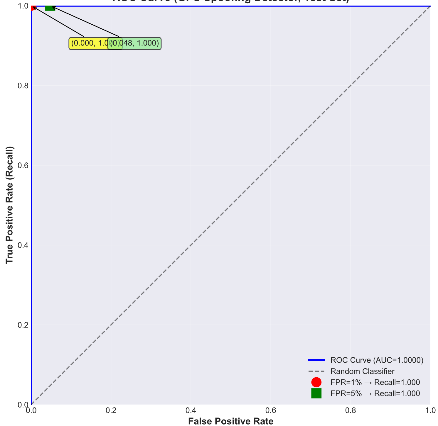
ROC Curve (GPS Spoofing Detector, Test Set)
