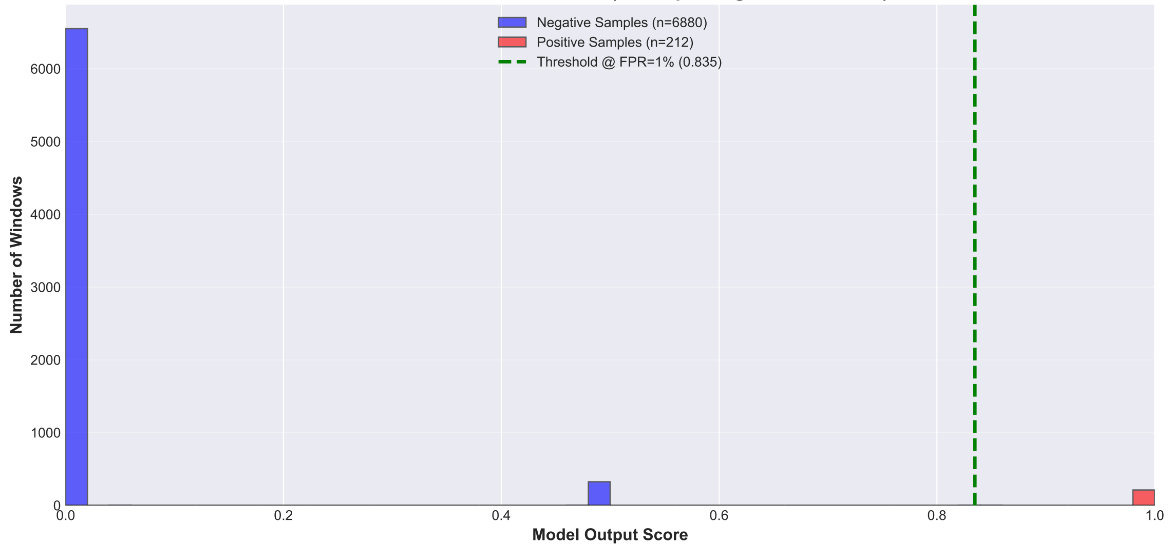
Score Distribution on Test Set (GPS Spoofing Detector, L=50)
