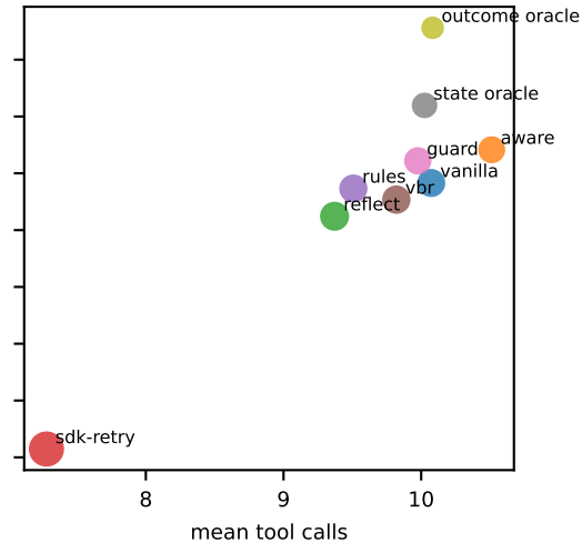
gemini-3.8-flash
