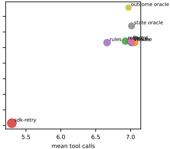
claude-opus-5.5
