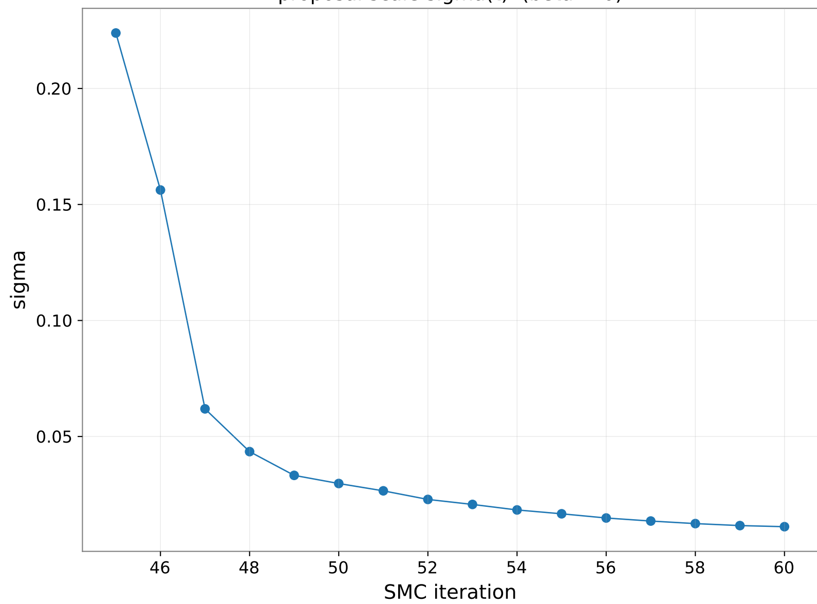
proposal scale sigma(t) (beta &gt; 0)
