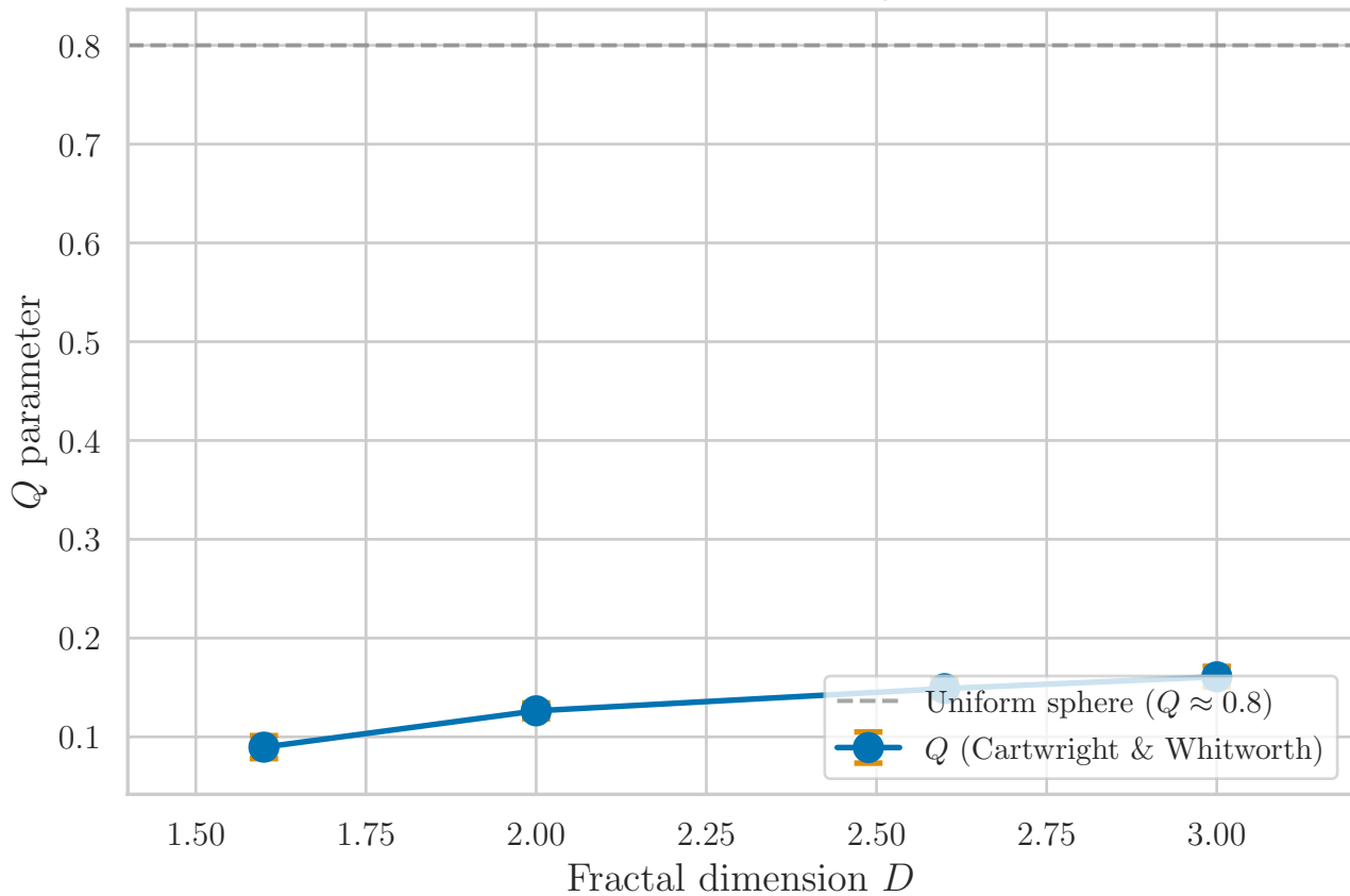
Fractal Substructure: Q vs D
