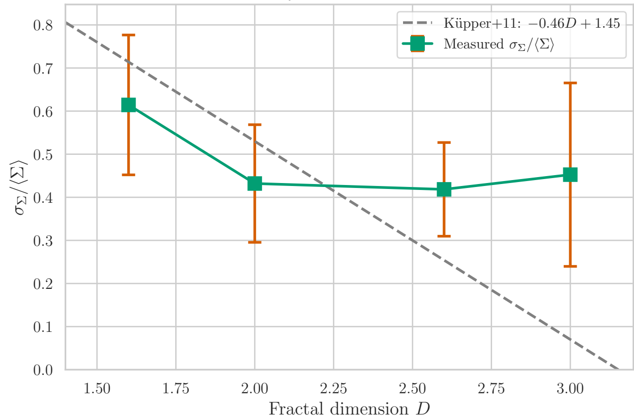
Azimuthal Density Variation vs Fractal Dimension
