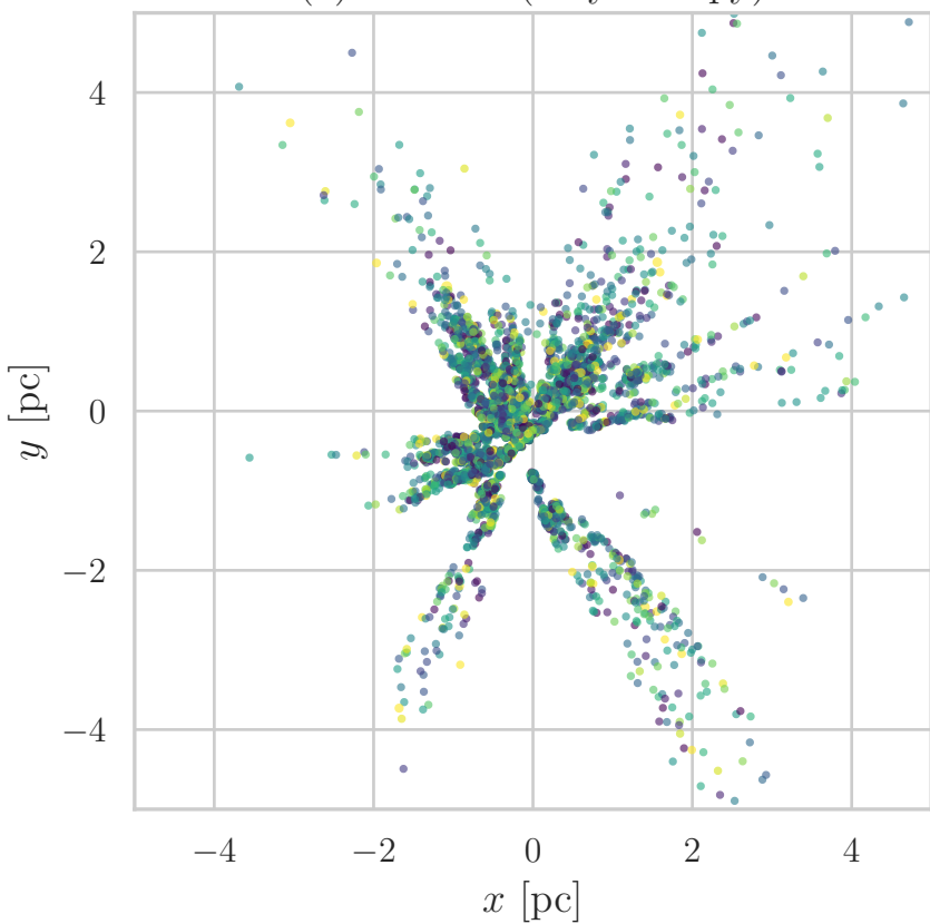
(c) D = 2.6 (weakly clumpy)
