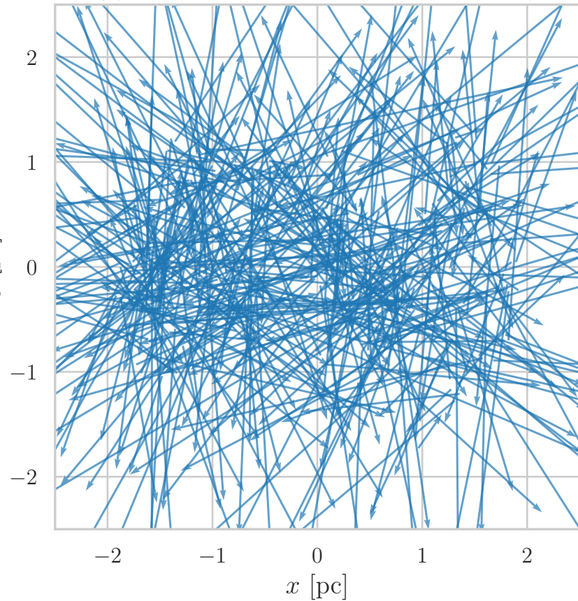
(a) Coherent velocities (ancestry-based)
