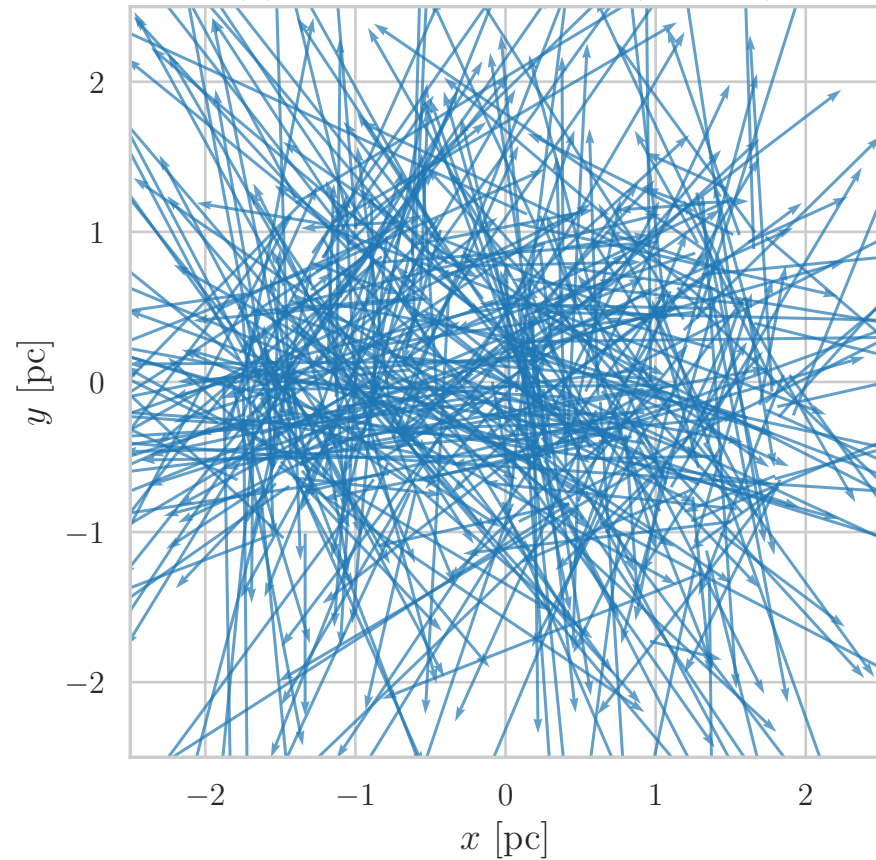
(b) Incoherent velocities (random)
