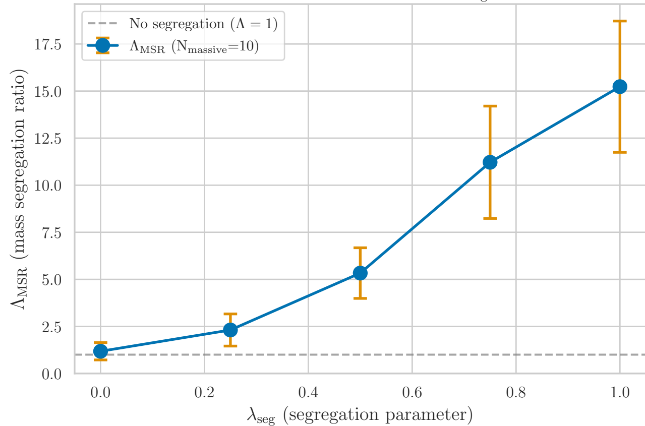
Mass Segregation: \Lambda_{\text{MSR}} vs \lambda_{\text{seg}}
