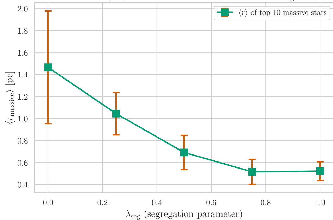
Mass Segregation: Mean Massive Star Radius vs \lambda_{\text{seg}}
