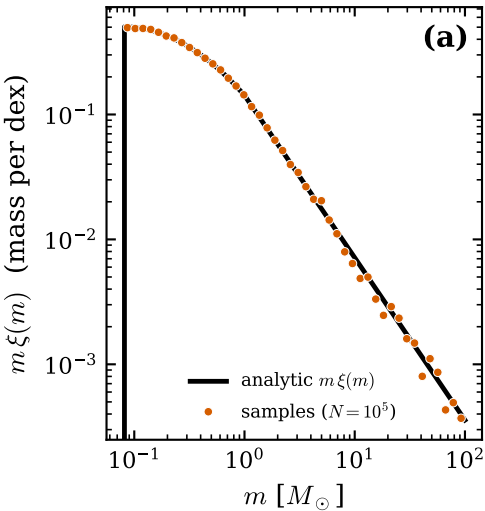
Chabrier (lognormal + PL)
