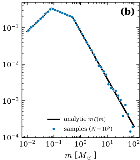
Kroupa (piecewise PL)
