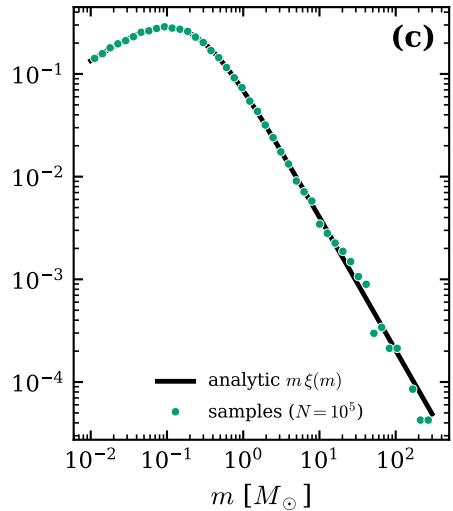
Maschberger (smooth)
