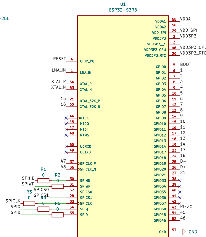
ESP32-S3R8
