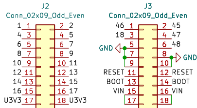
Headers
