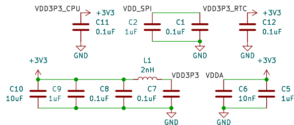
MCU power
