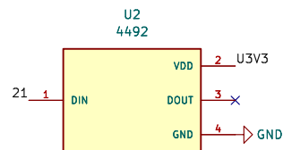
RGB LED
