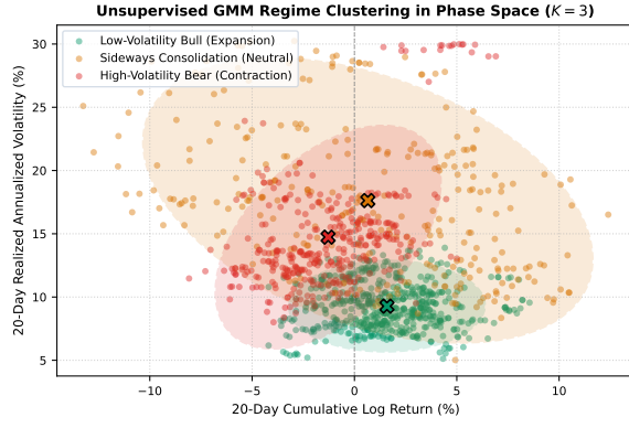
Fig. 2. Unsupervised Gaussian Mixture Model ( K = 3 ) clustering in phase space. The 95% confidence ellipses and centroid markers (X) demonstrate clear structural bifurcation between Low-Volatility Bull, Sideways Consolidation, and High-Volatility Bear regimes.
