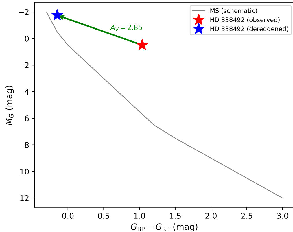
Colour-Magnitude Diagram
