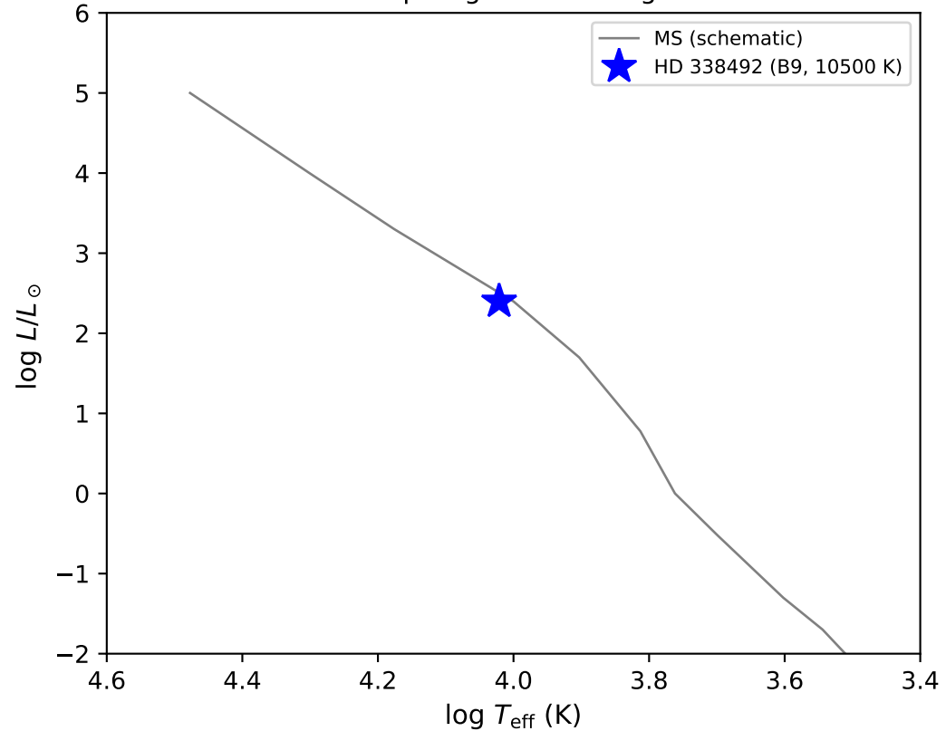
Hertzsprung-Russell Diagram
