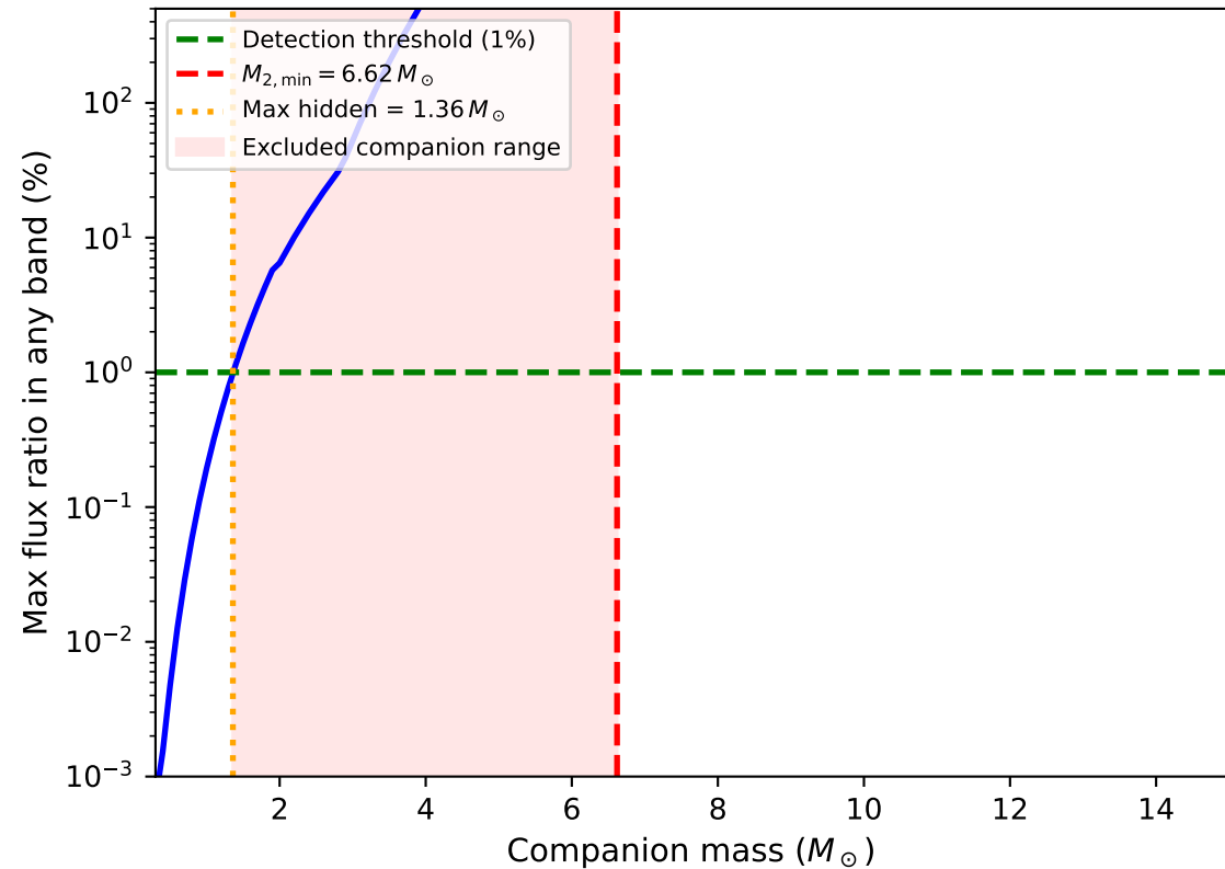
Companion detectability vs mass
