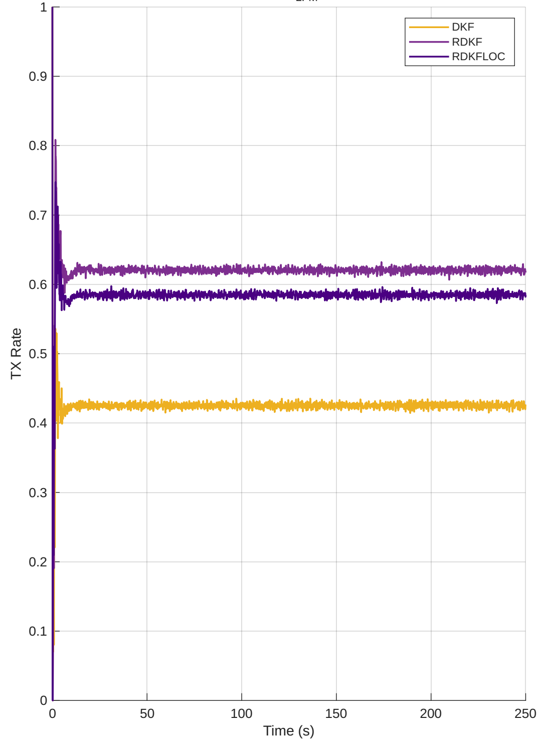
TX Rate vs Time — DKF vs RDKF vs RDKFLOC (LFM data) b = 0.005 , b_{\text{LFM}} = 0.01
