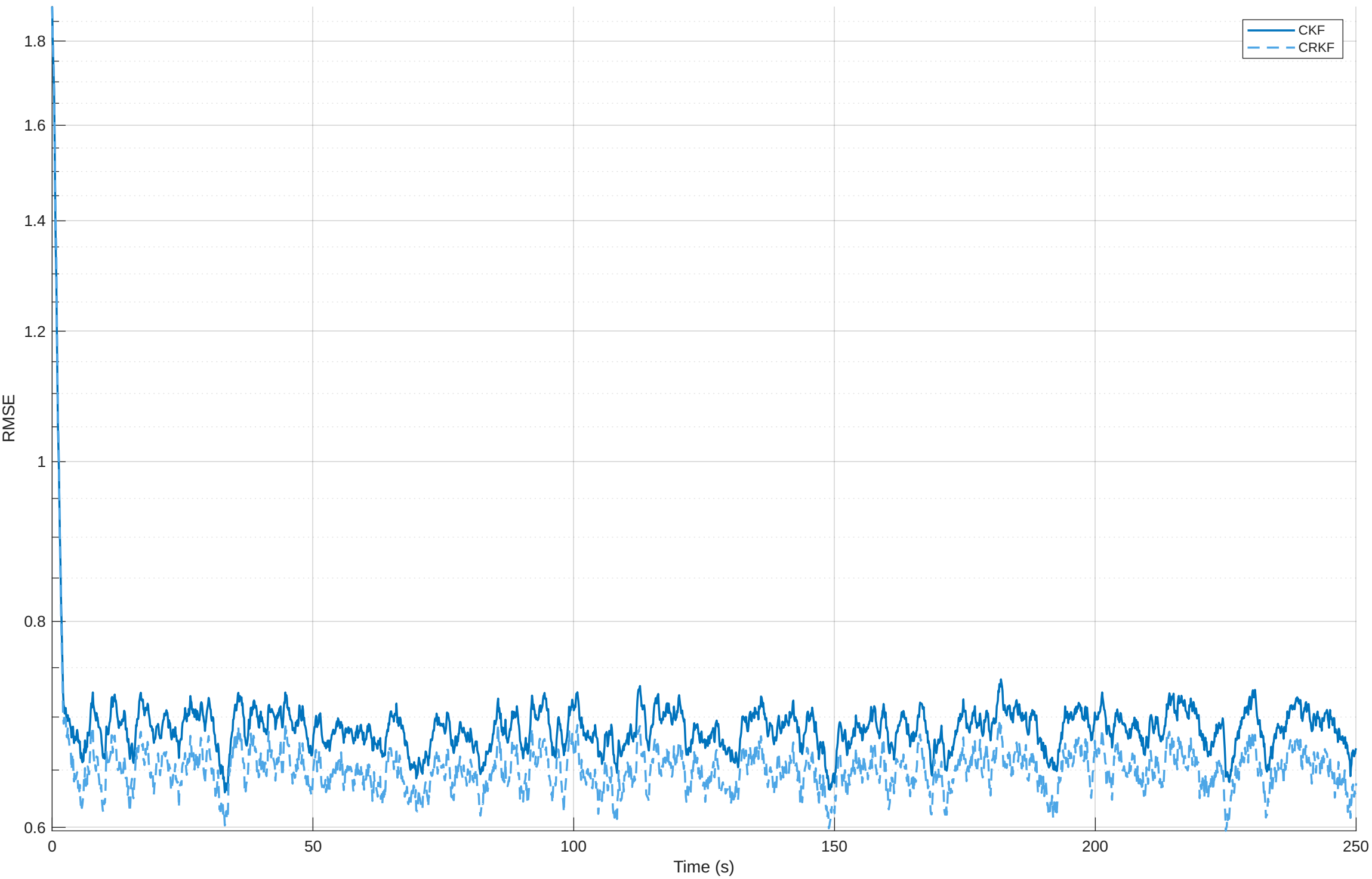
RMSE vs Time — CKF vs CRKF (LFM data) b = 0.005, b_{\text{LFM}} = 0.01
