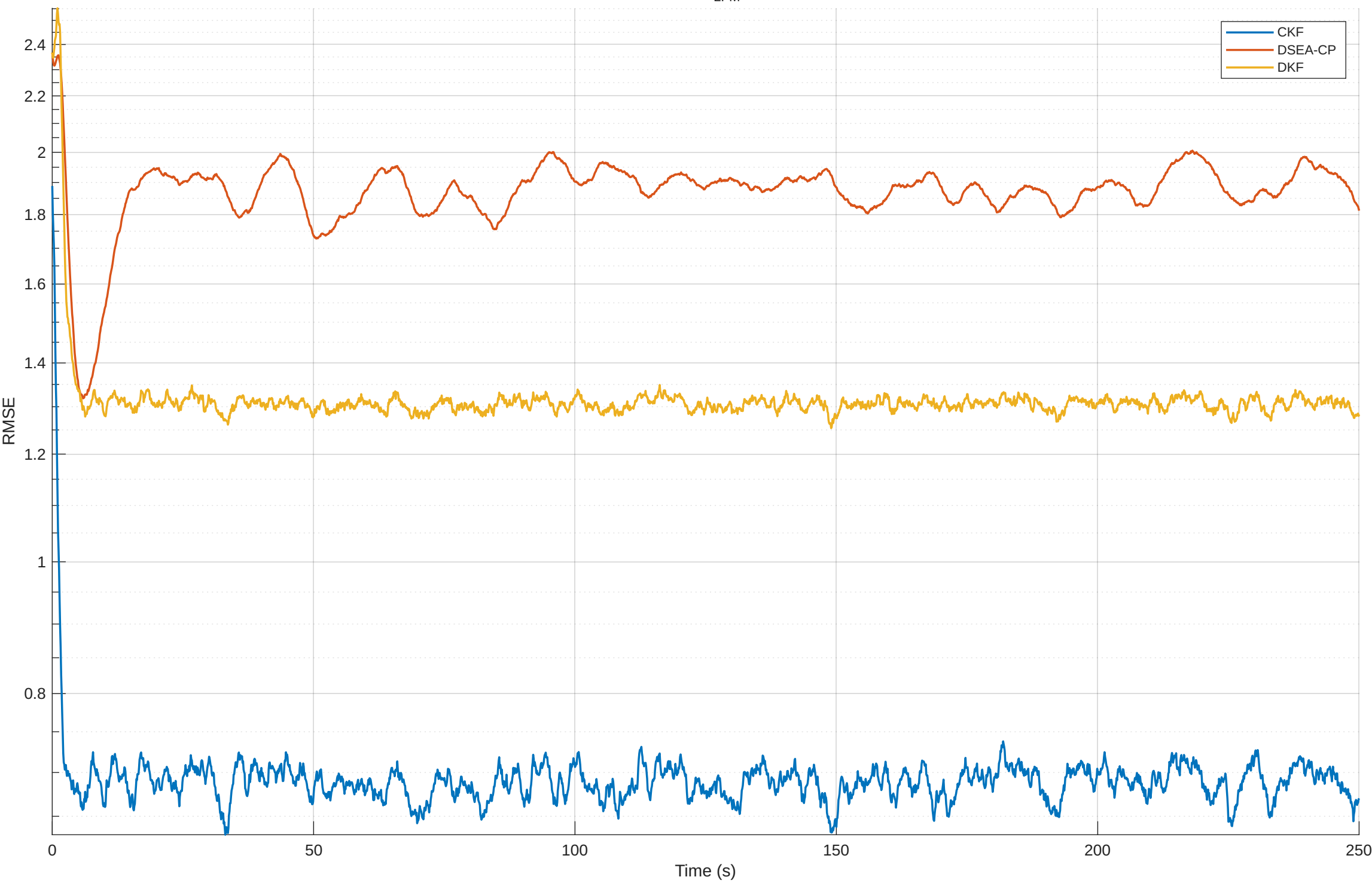
RMSE vs Time — CKF vs DSEA-CP vs DKF (LFM data)
