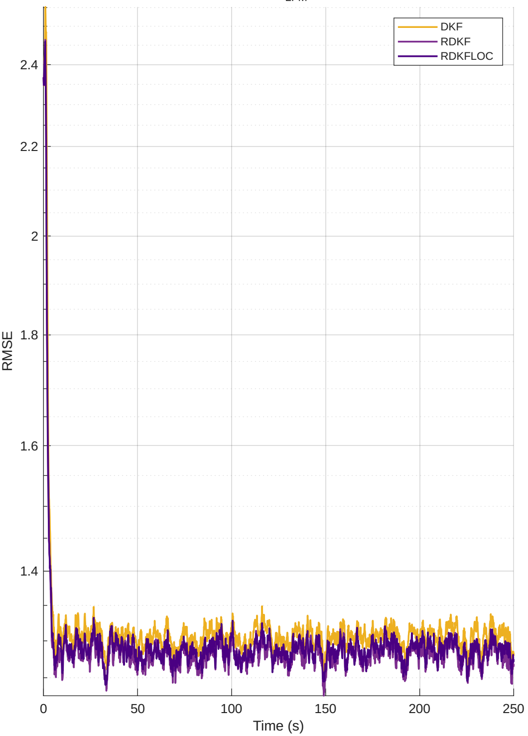
RMSE vs Time — DKF vs RDKF vs RDKFLOC (LFM data) b = 0.005 , b_{\text{LFM}} = 0.01
