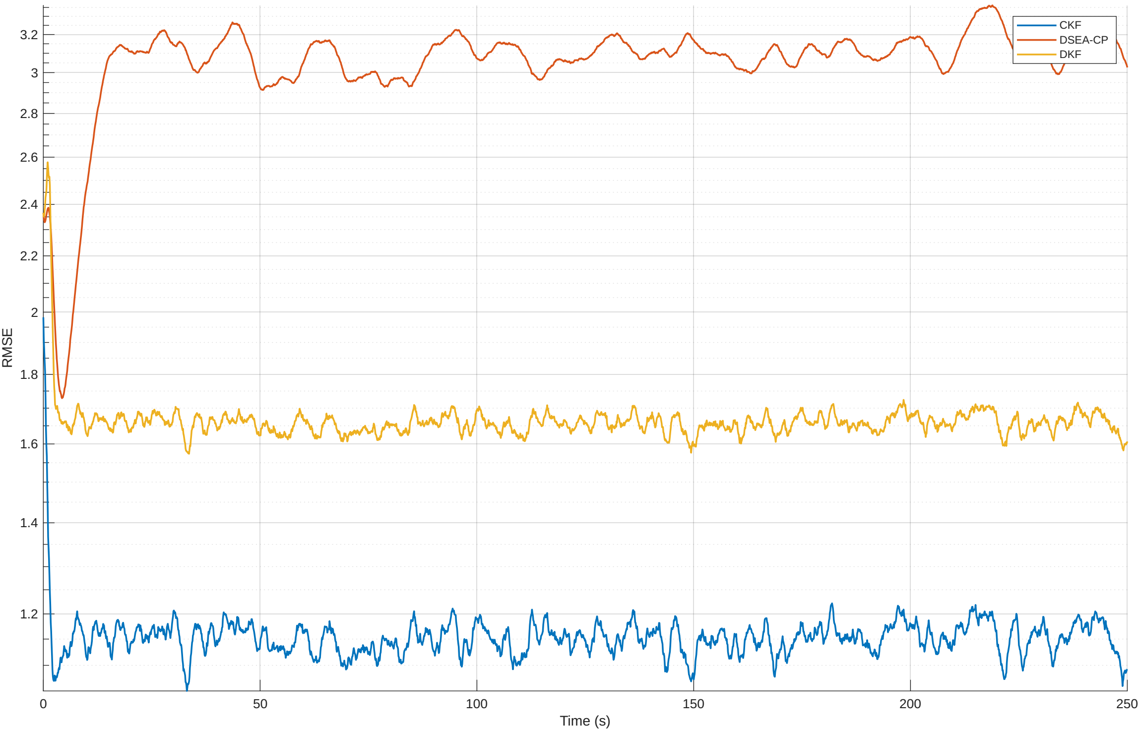
RMSE vs Time — CKF vs DSEA-CP vs DKF (LFM data) b = 0.005 , b_{\text{LFM}} = 0.05
