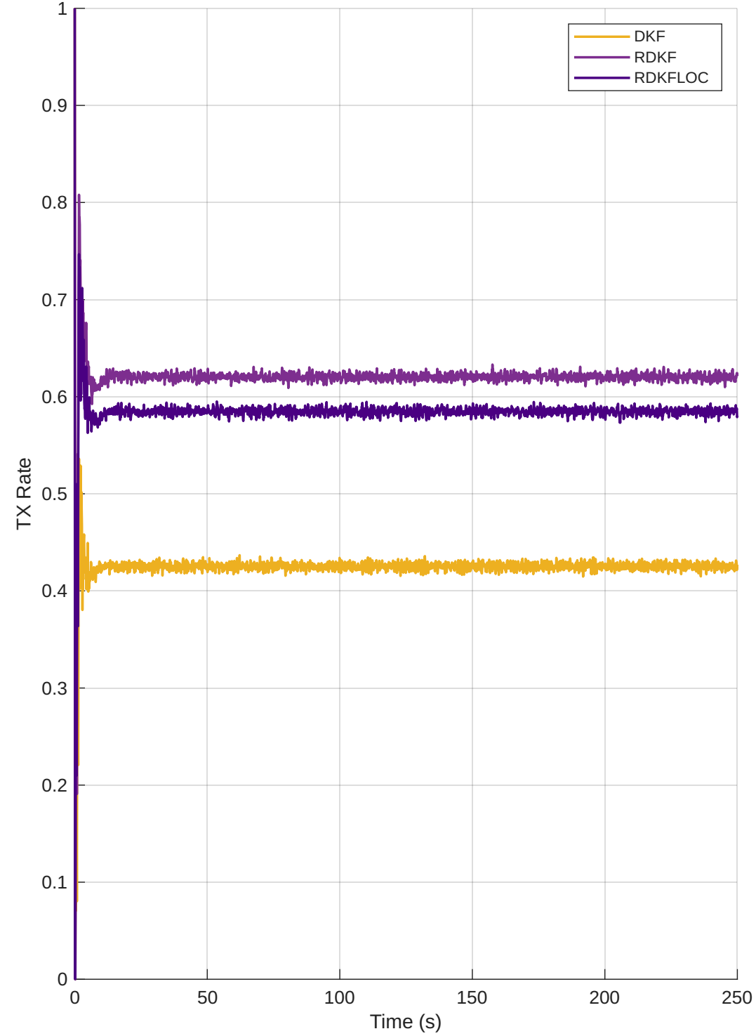
TX Rate vs Time — DKF vs RDKF vs RDKFLOC (LFM data) b = 0.005 , b_{\text{LFM}} = 0.05
