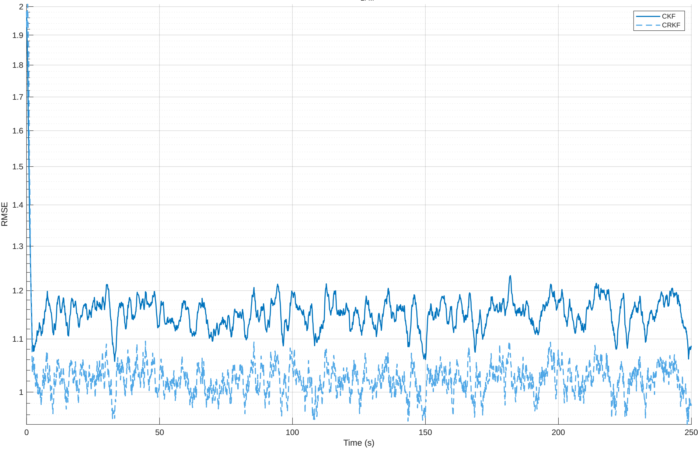
RMSE vs Time — CKF vs CRKF (LFM data) b = 0.05 , b_{\text{LFM}} = 0.05
