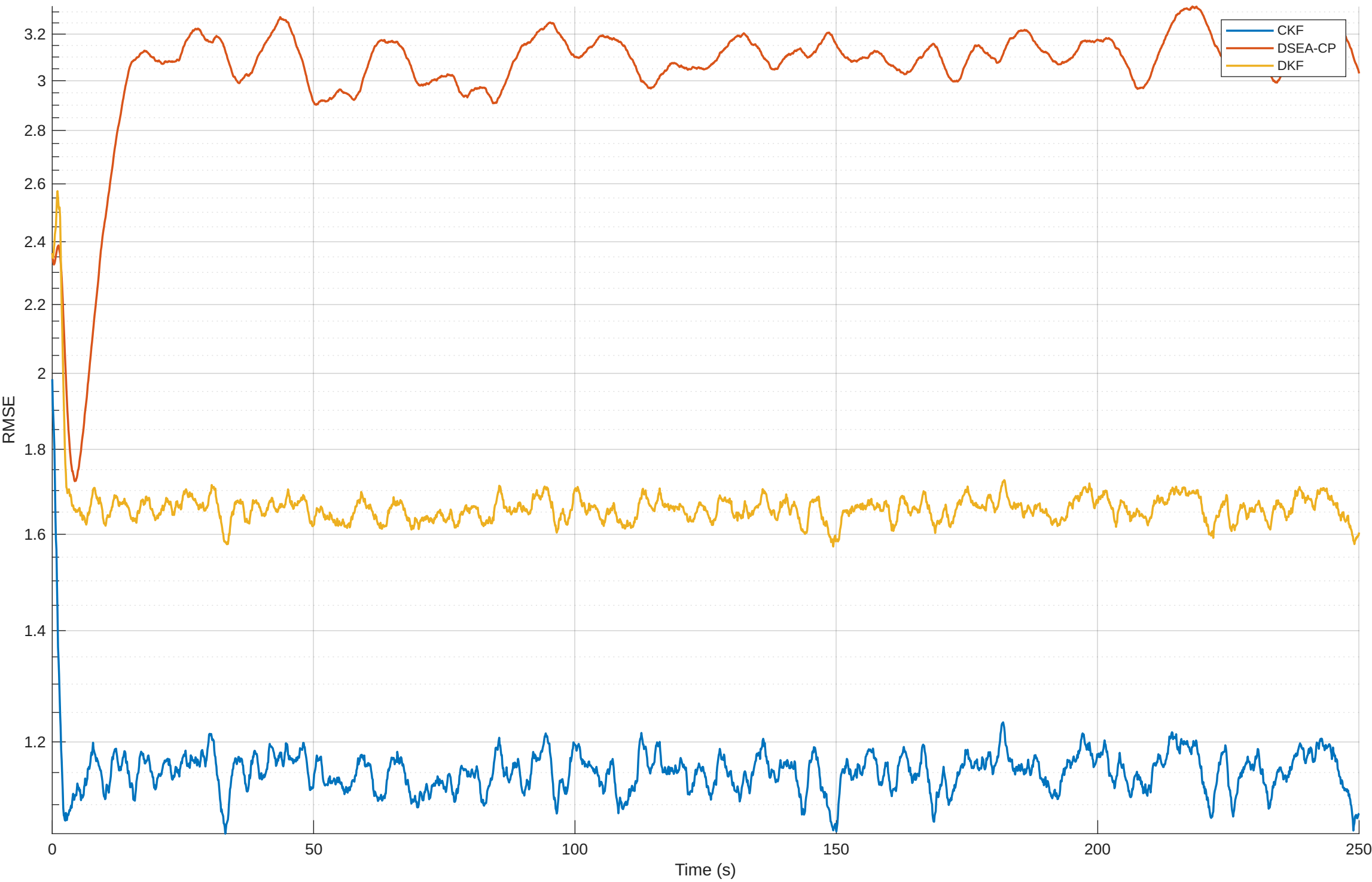
RMSE vs Time — CKF vs DSEA-CP vs DKF (LFM data) b = 0.05 , b_{\text{LFM}} = 0.05
