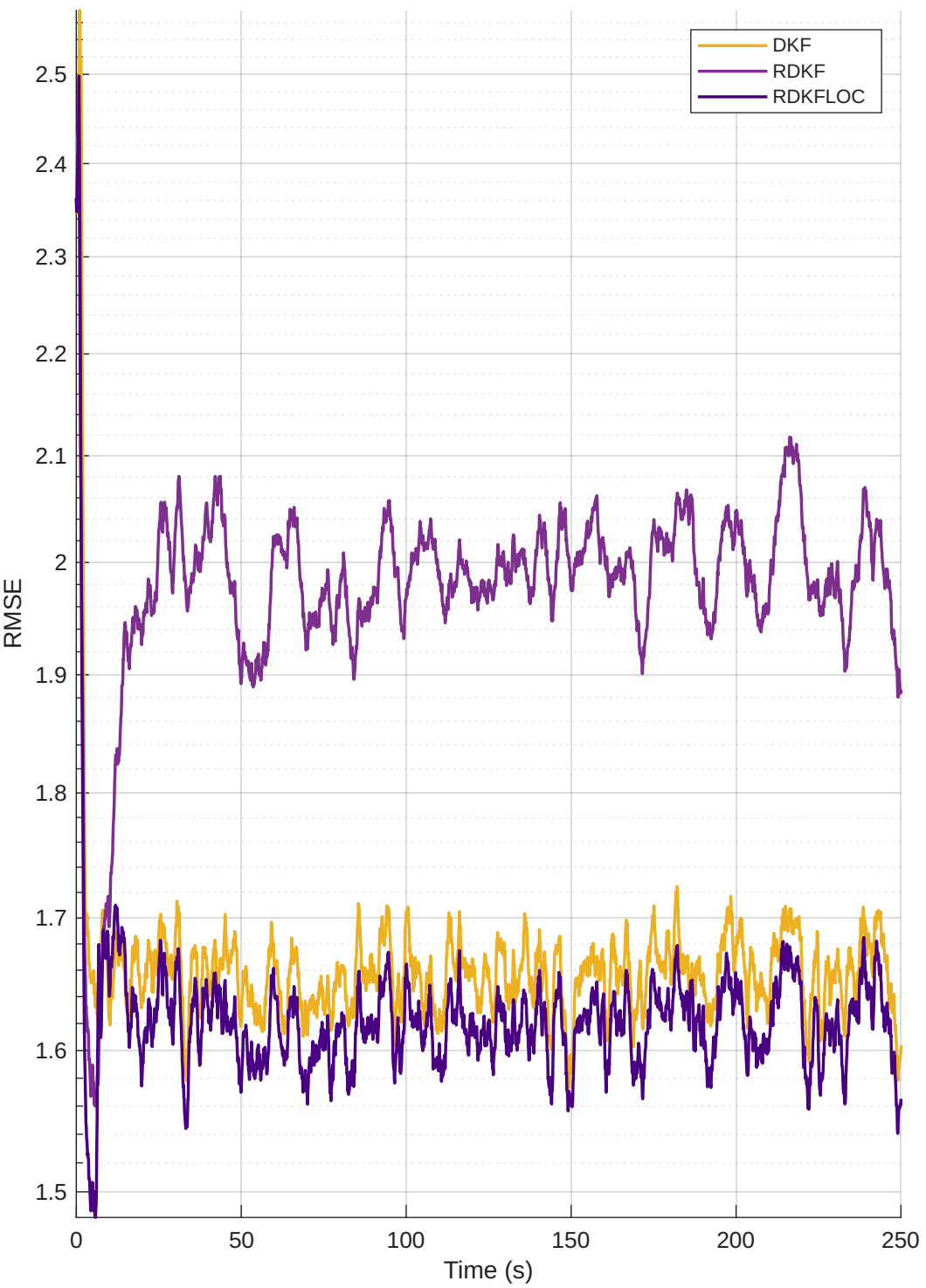
RMSE vs Time — DKF vs RDKF vs RDKFLOC (LFM data) b = 0.05, b_{\text{LFM}} = 0.05
