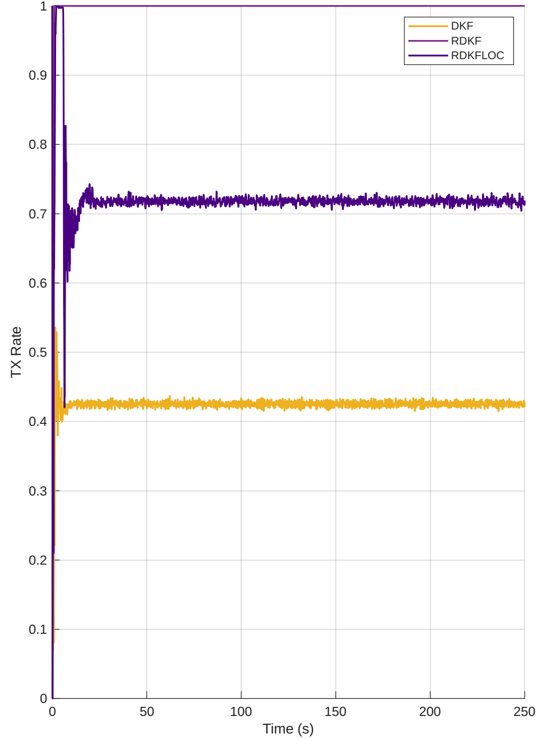
TX Rate vs Time — DKF vs RDKF vs RDKFLOC (LFM data) b = 0.05, b_{\text{LFM}} = 0.05
