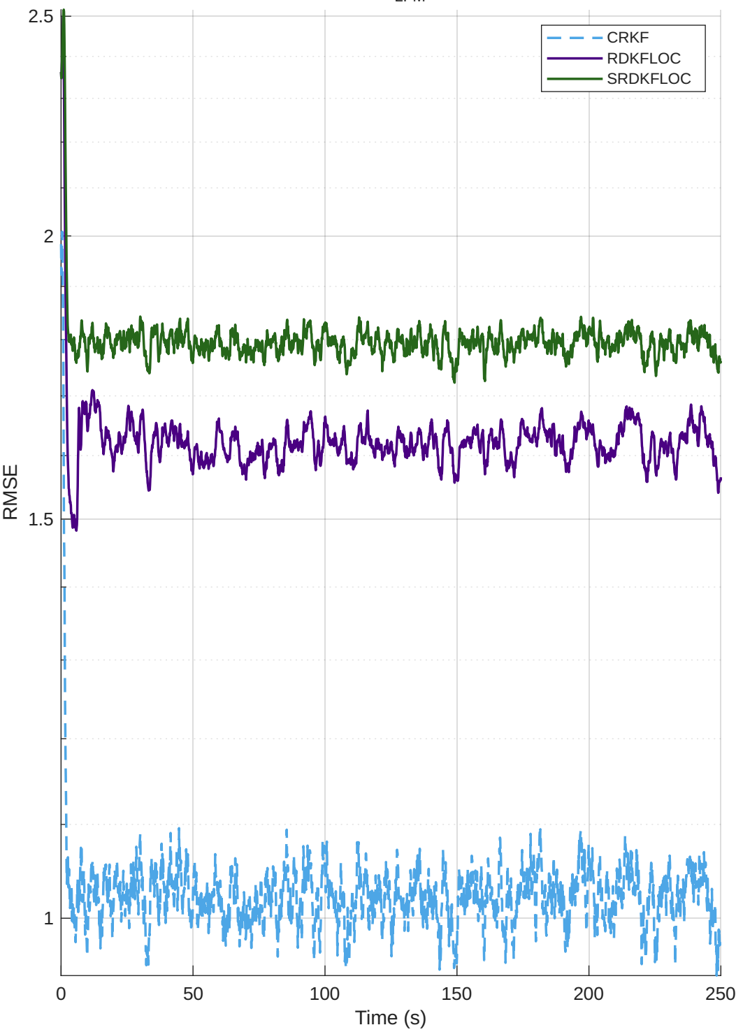
RMSE vs Time — CRKF vs RDKFLOC vs SRDKFLOC (LFM data) b = 0.05, b_{\text{LFM}} = 0.05
