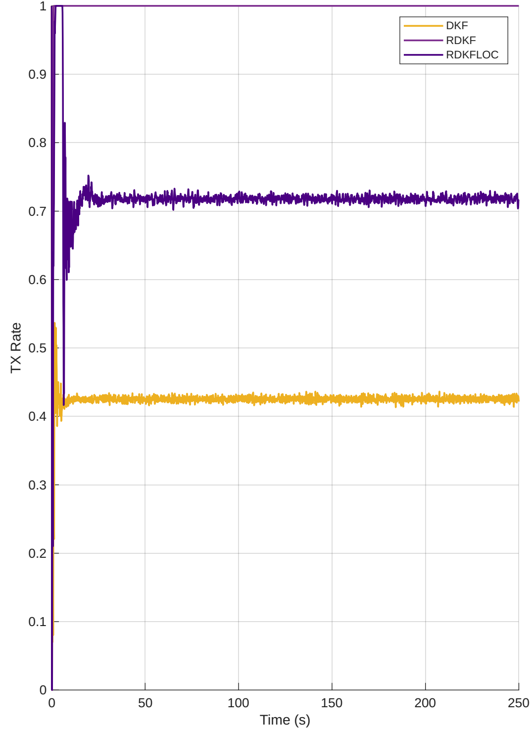
TX Rate vs Time — DKF vs RDKF vs RDKFLOC b = 0.05, b_{\text{LFM}} = 0.05
