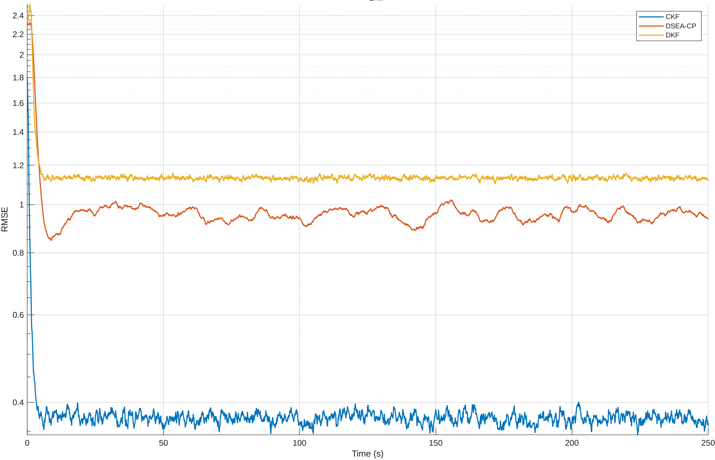
RMSE vs Time — CKF vs DSEA-CP vs DKF b = 0.05 , b_{\text{LFM}} = 0.05
