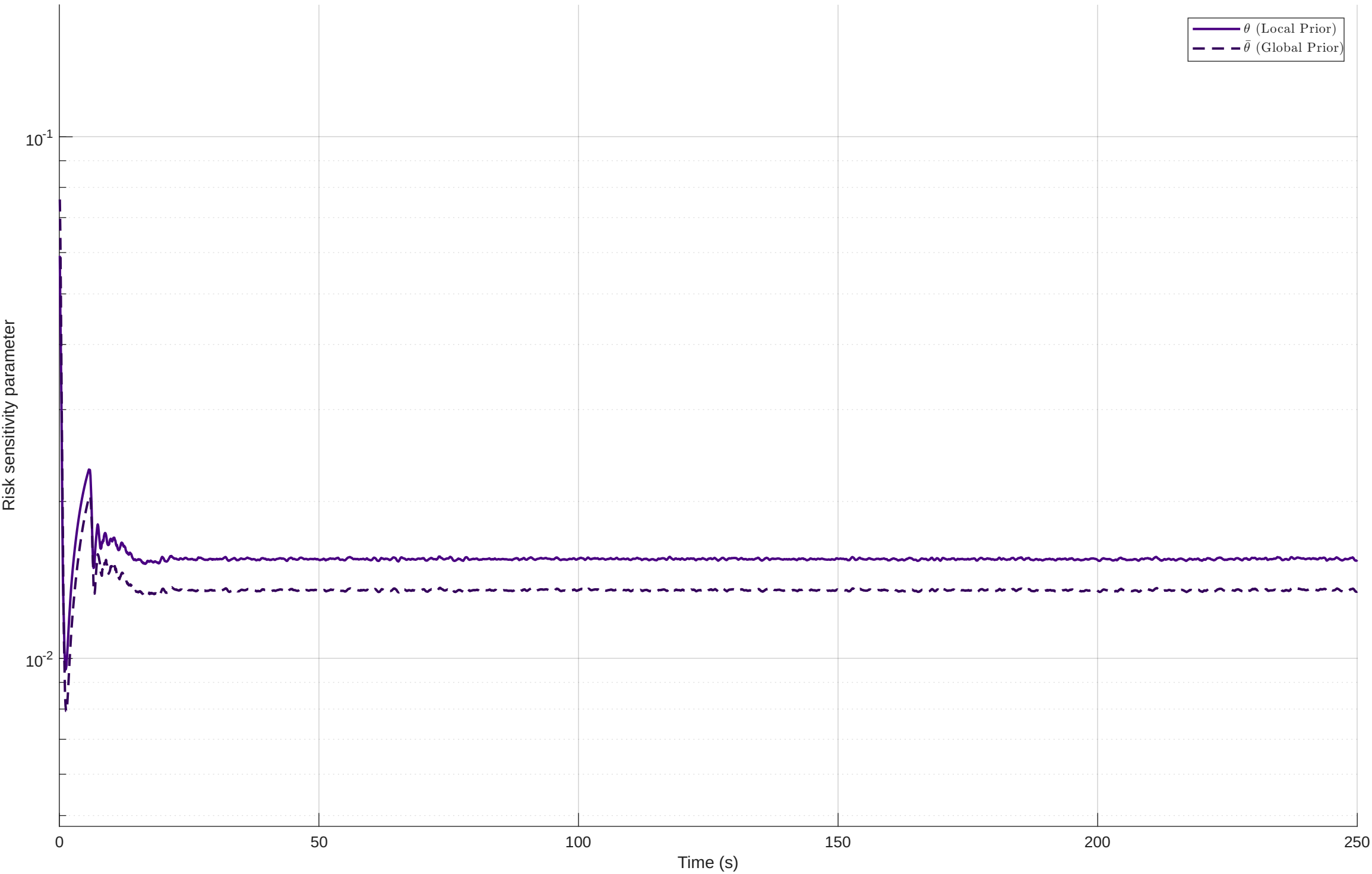
Risk Sensitivity \theta vs \bar{\theta} - RDKFLOC
