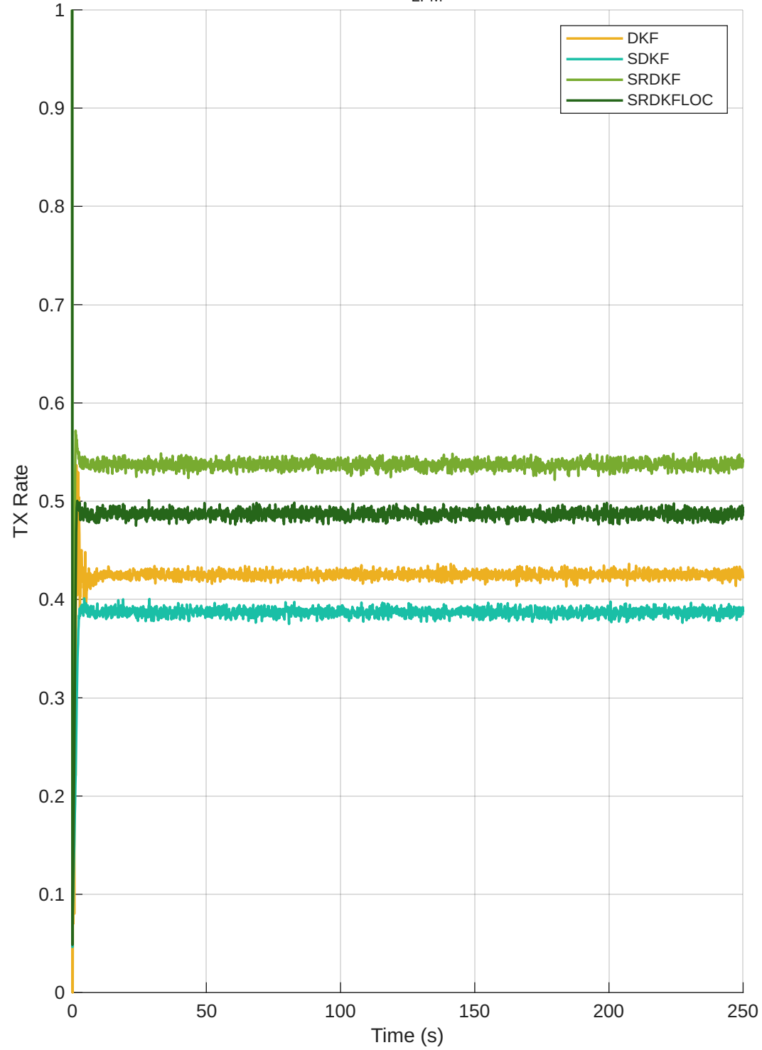
TX Rate vs Time — DKF vs SDKF vs SRDKF vs SRDKFLOC b = 0.05 , b_{\text{LFM}} = 0.05
