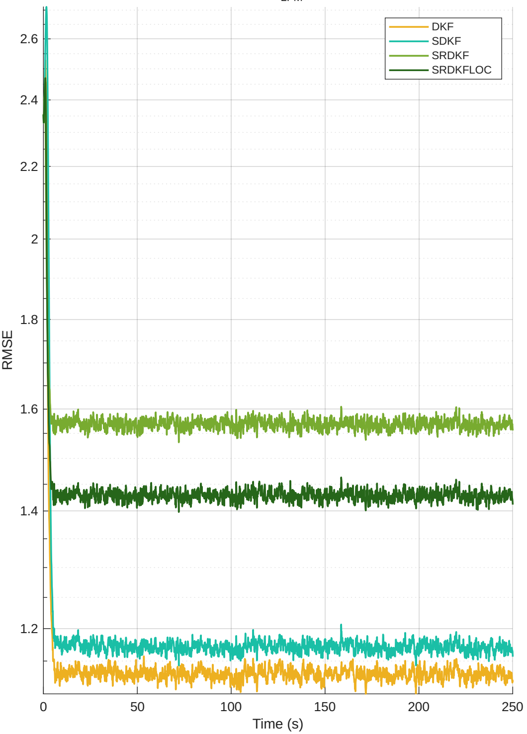
RMSE vs Time — DKF vs SDKF vs SRDKF vs SRDKFLOC b = 0.05 , b_{\text{LFM}} = 0.05
