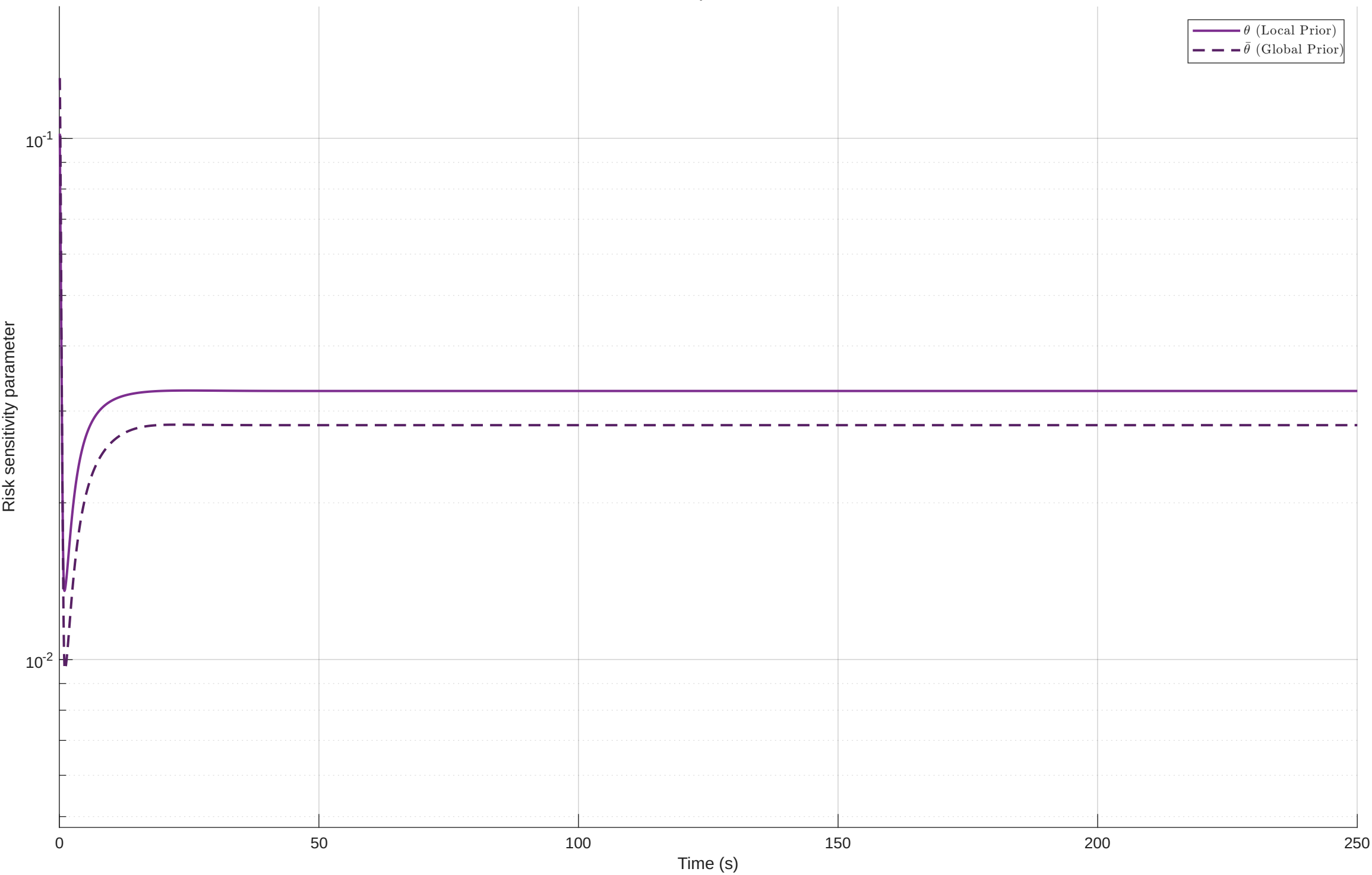
Risk Sensitivity \theta vs \bar{\theta} - RDKF
