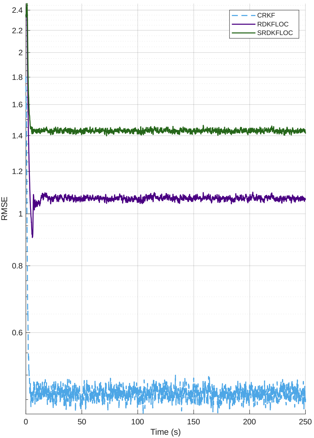
RMSE vs Time — CRKF vs RDKFLOC vs SRDKFLOC b = 0.05, b_{\text{LFM}} = 0.05
