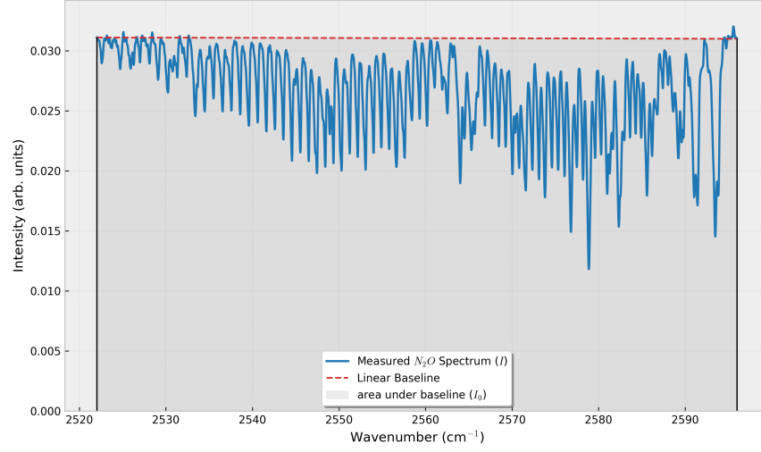
Figure 11: N_2O Band at 2522 to 2596 cm^{-1}
