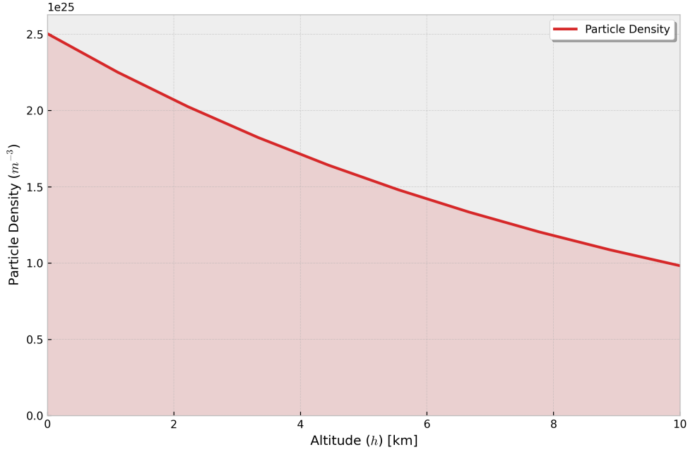
Figure 10: Particle density vs. Altitude
