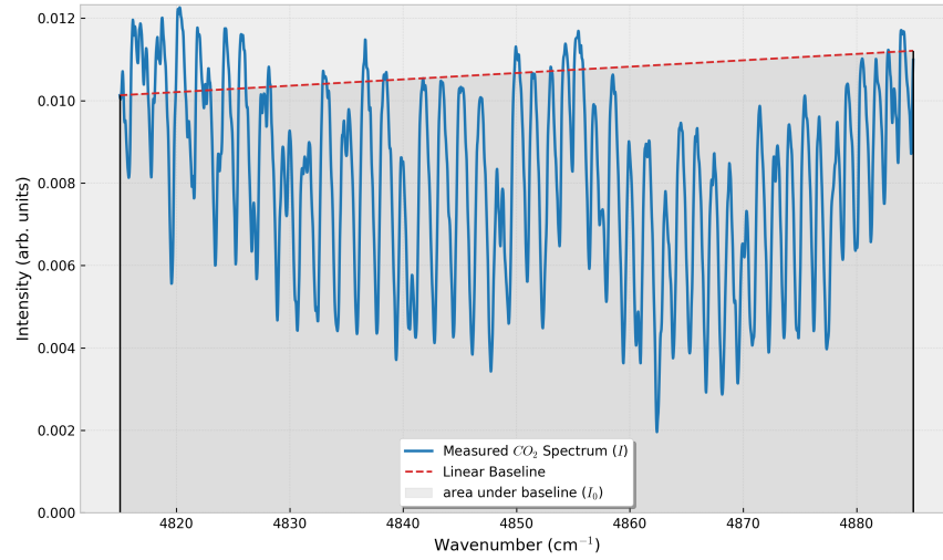
Figure 12: CO_2 Band at 4815 to 4885 cm^{-1}
