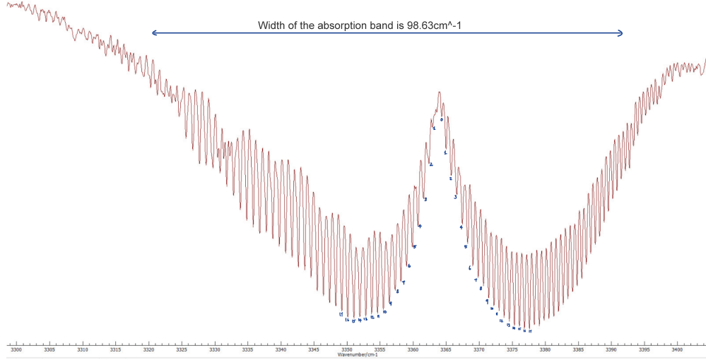
Figure 8: N_2O absorption band with J_{max} .
