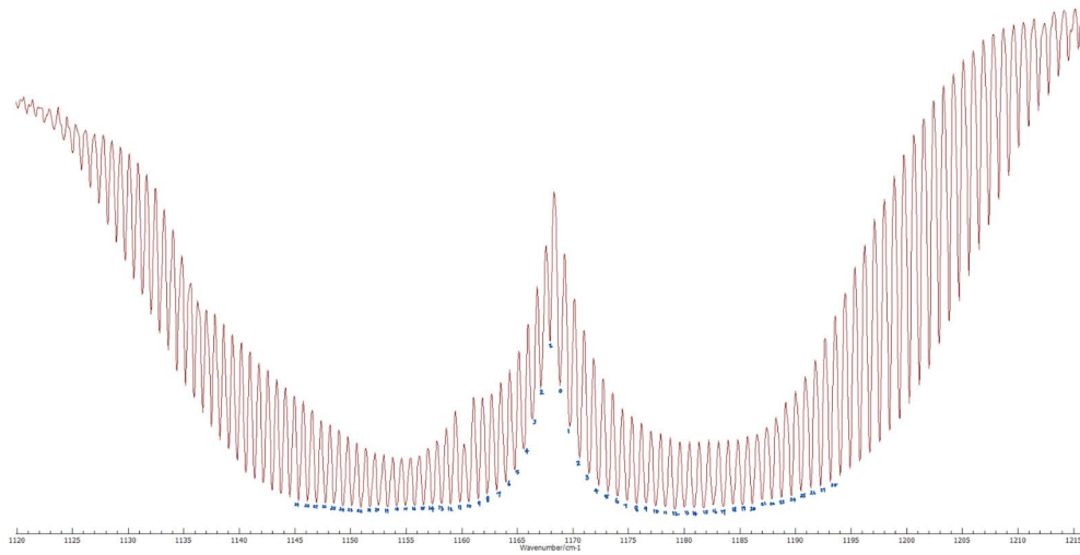
Figure 9: N_2O absorption band with J_{max} .
