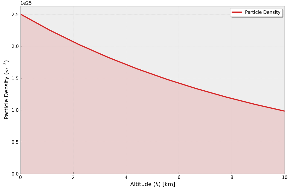
Figure 10: Particle density vs. Altitude
