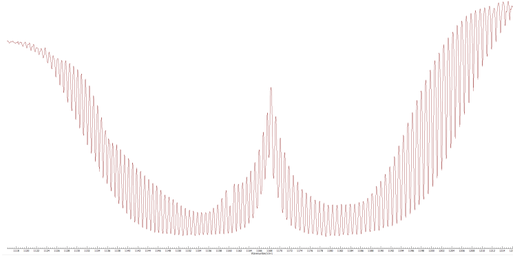
Figure 6: N_2O Absorption bands chosen for moment of inertia calculation.
