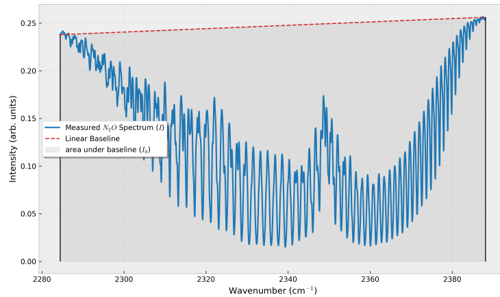
Figure 7: N_2O Absorption bands chosen for gas pressure calculation.
