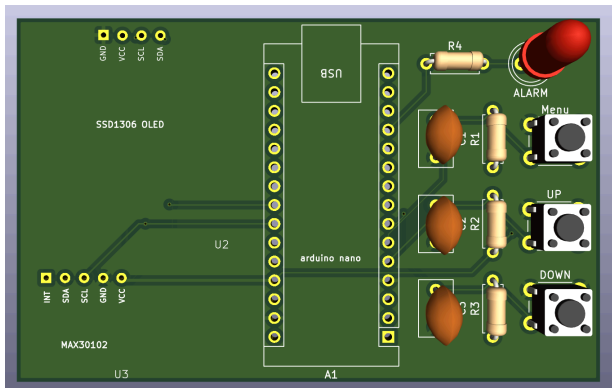
PCB heart rate monitor:
