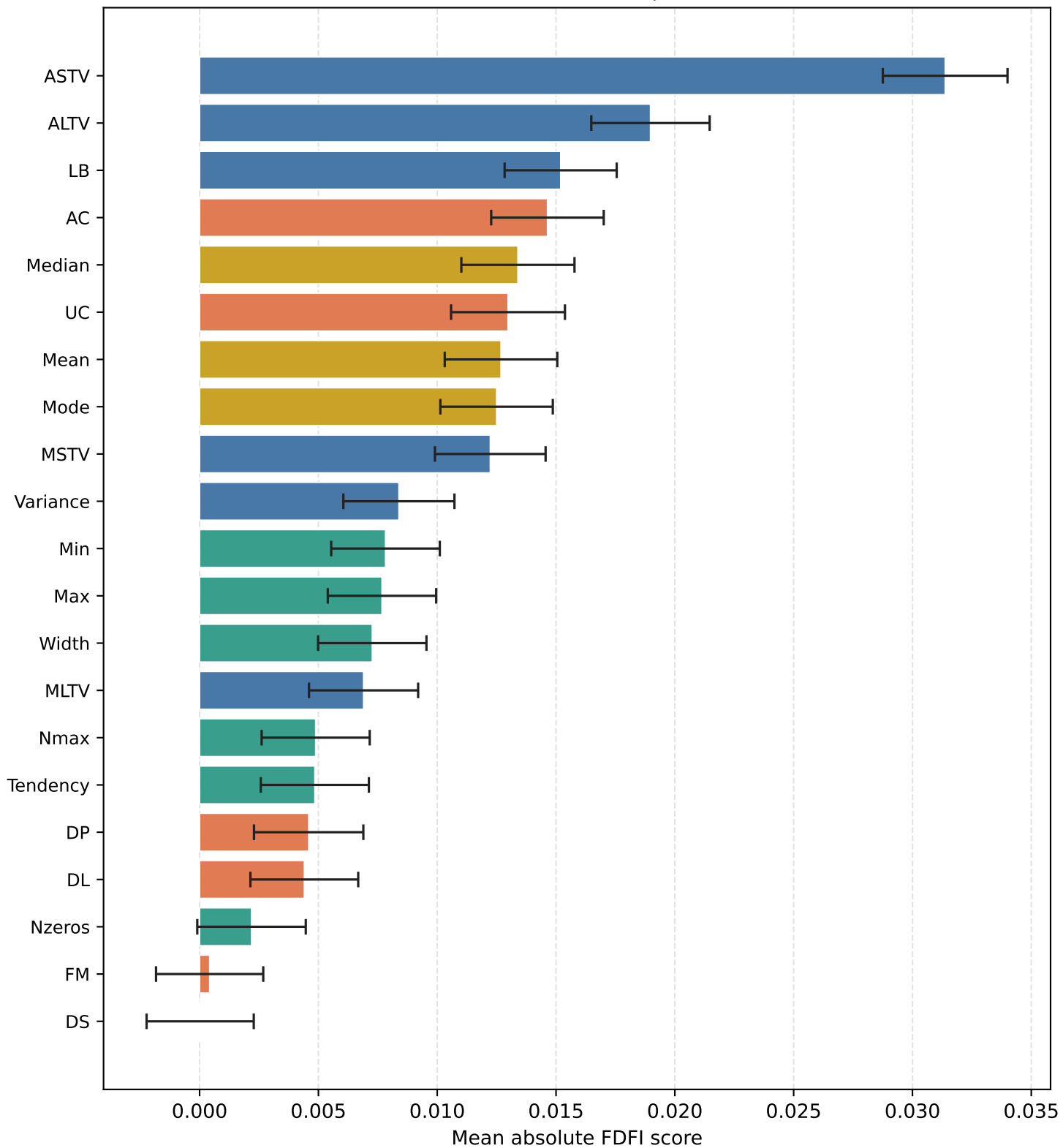
Global FDFI Feature Importance
