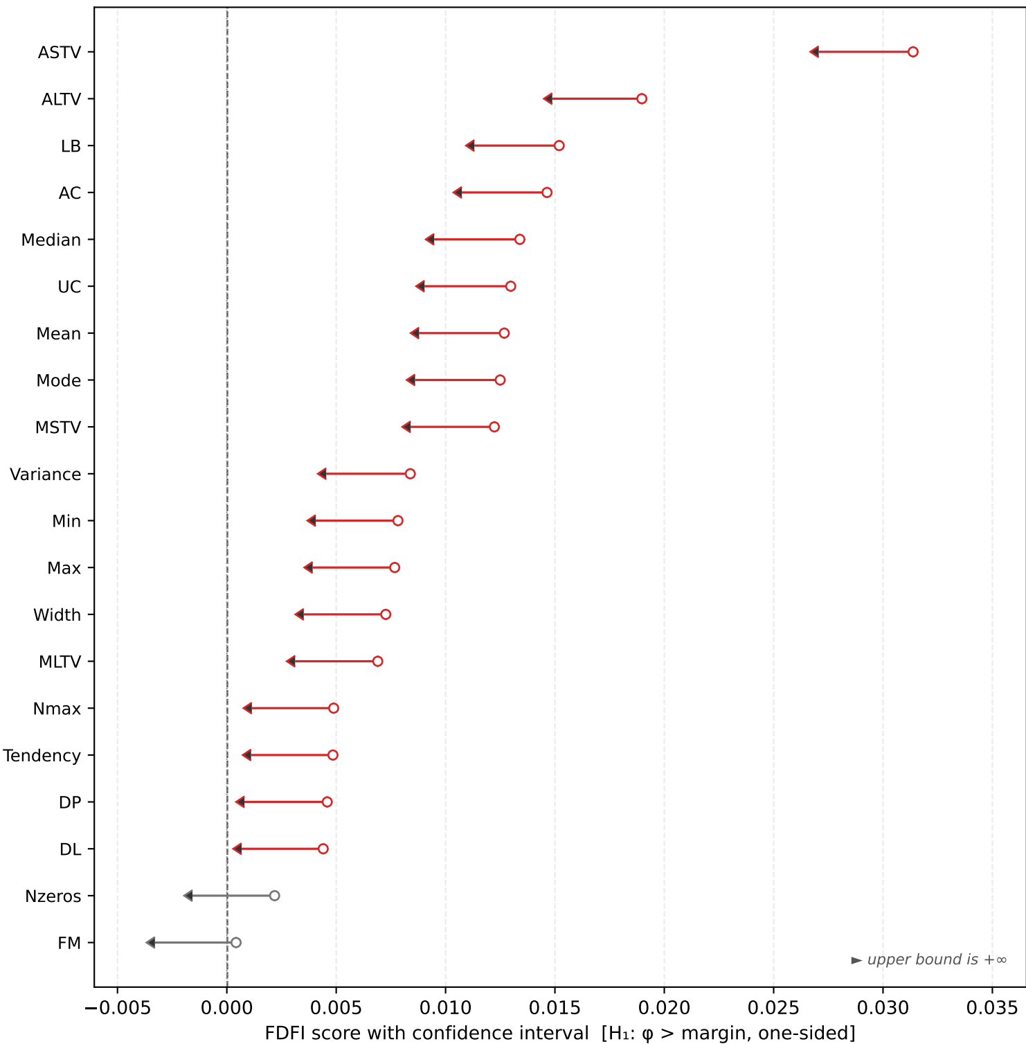
FDFI Confidence Intervals (one-sided)
