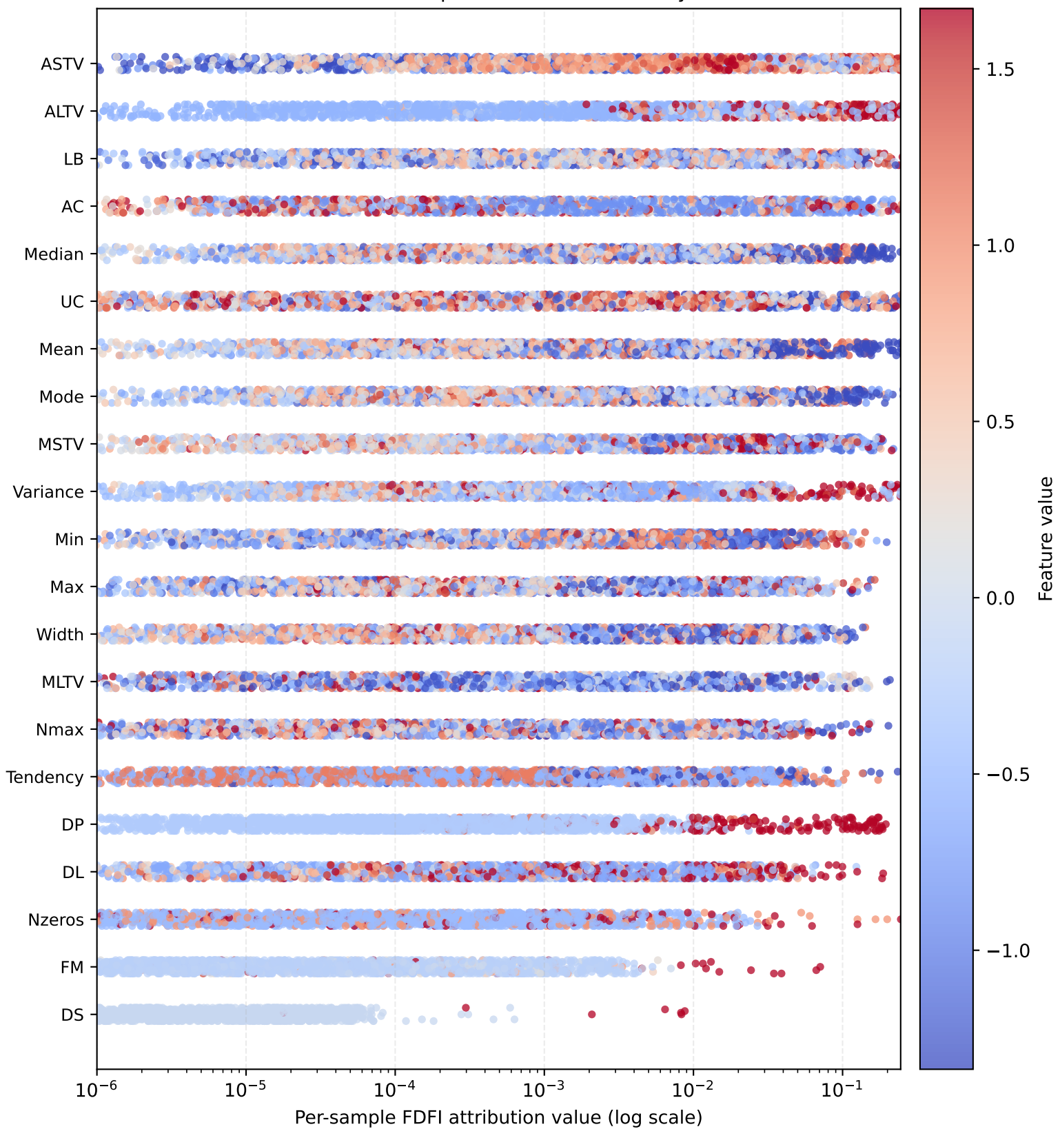
FDFI Per-sample Attribution Summary
