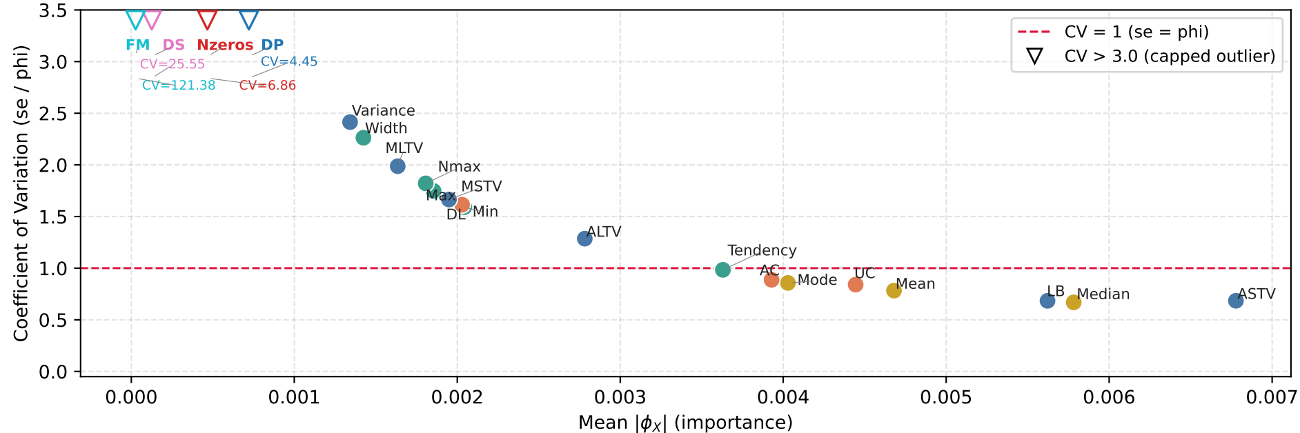
Attribution Reliability: Importance vs. Coefficient of Variation (Note: Features with CV > 3.0 are capped at the top edge)
