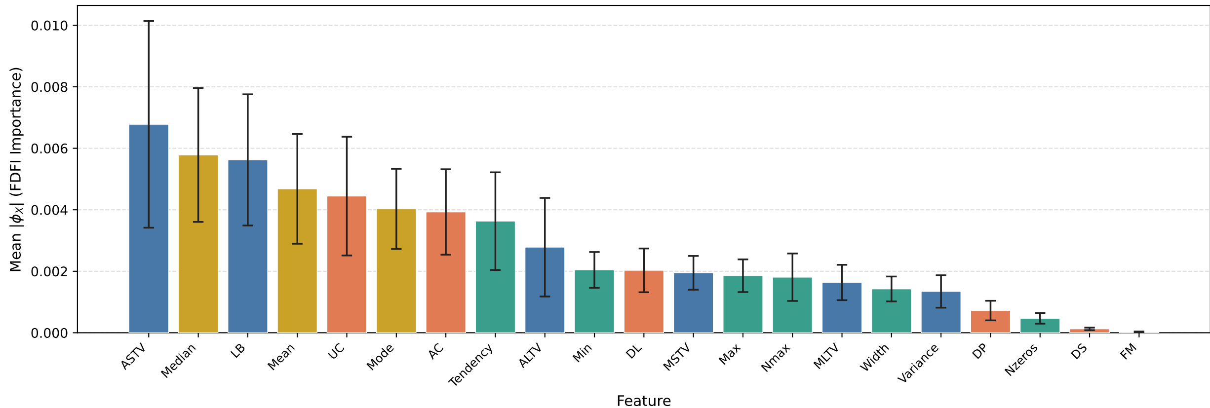
Global FDFI Feature Importance with Uncertainty Quantification (Error bars = bootstrap standard error; features sorted by decreasing importance)
