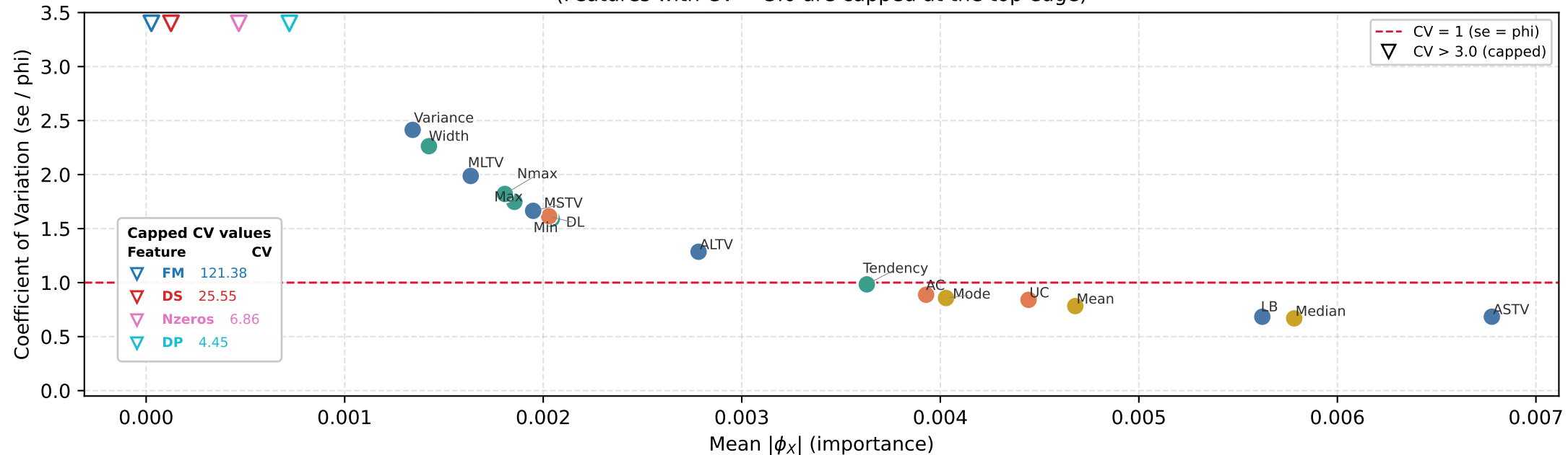
Attribution Reliability: Importance vs. Coefficient of Variation (Features with CV > 3.0 are capped at the top edge)
