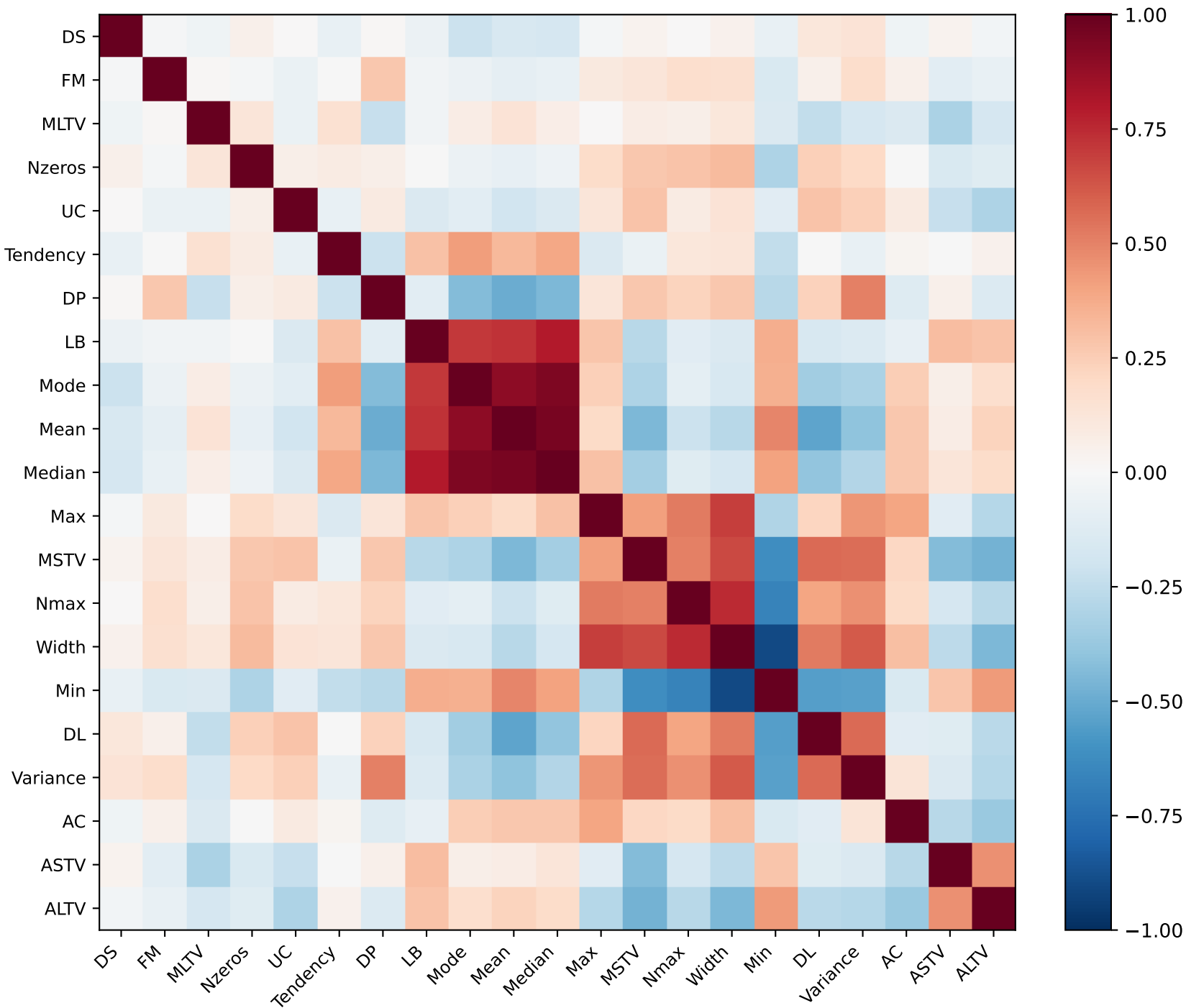
Pearson Correlation Matrix — Feature Space (Hierarchical-clustering reordering reveals collinear blocks)
