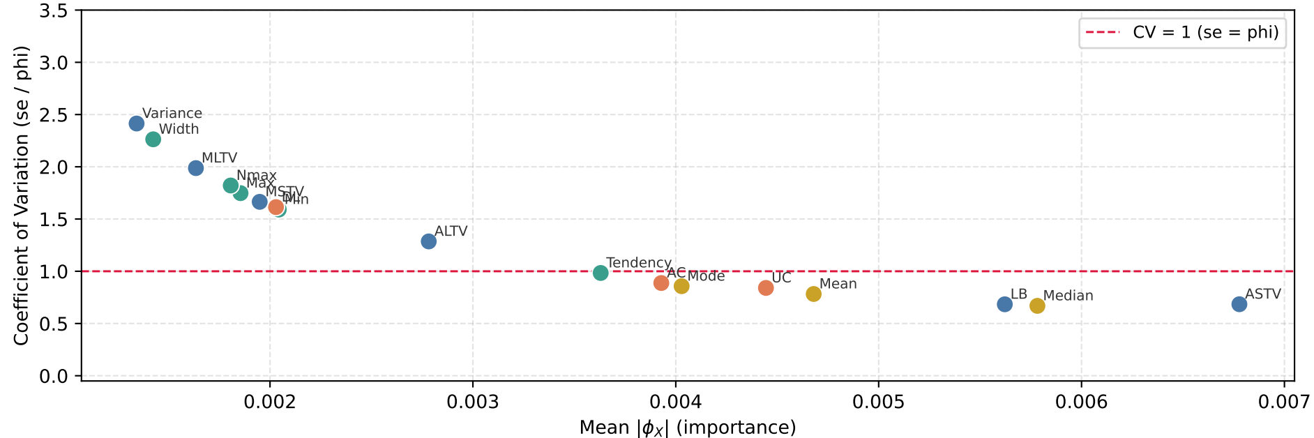
Attribution Reliability: Importance vs. Coefficient of Variation (Note: Features with CV > 3.0 excluded for visual clarity)
